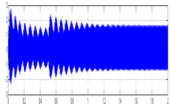
Fig 3.4: PI controlled CF3AS Output current
