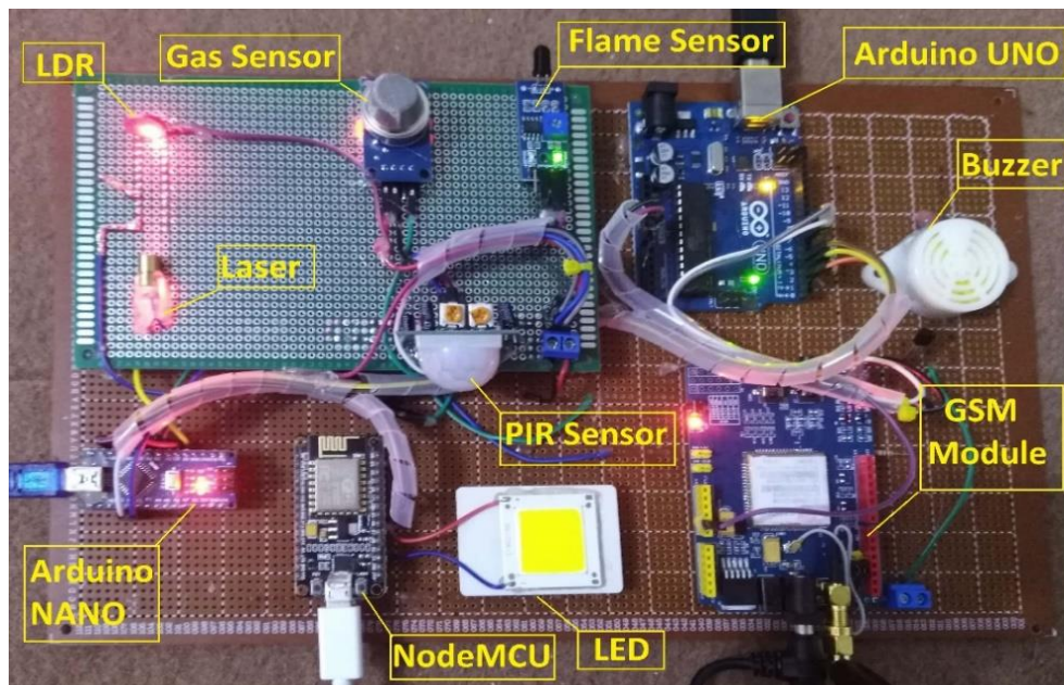
Fig. 12: The Implemented Safety and Security System.
