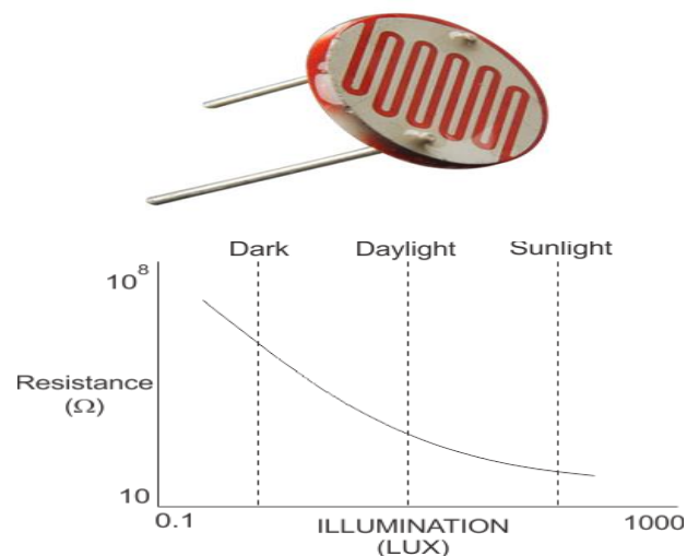
Fig. 8: The Light Dependent Resistance.
