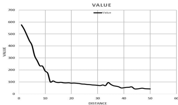
Fig. 5: Flame Sensor Output vs. Distance.
