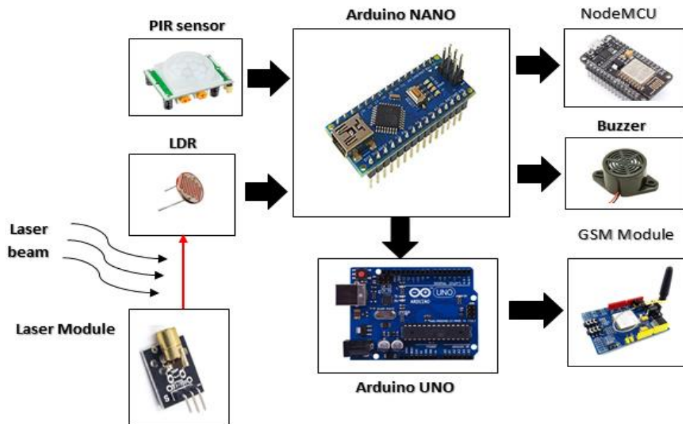
Fig. 10: Block Diagram of Security Part.
