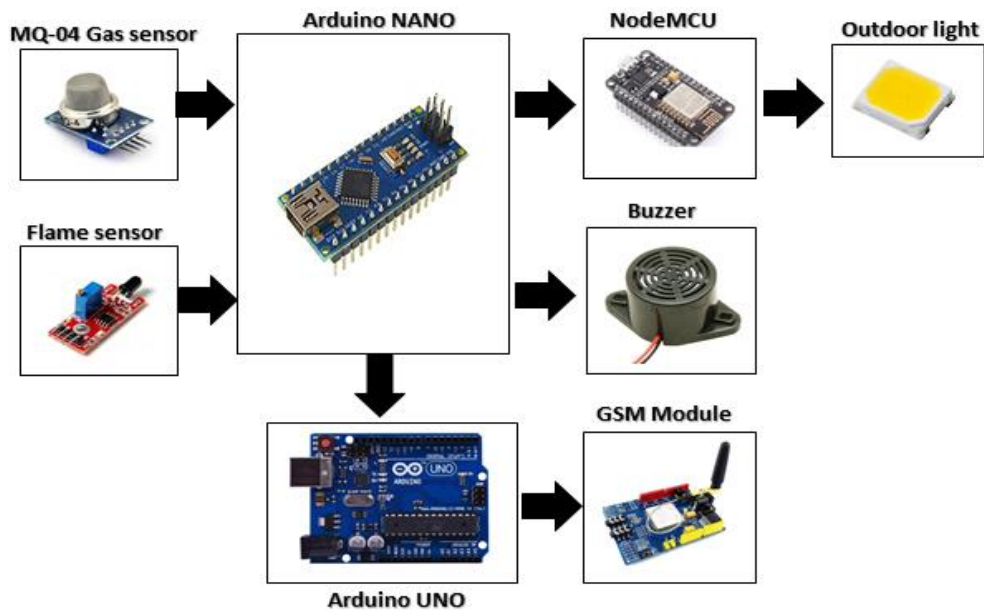
Fig. 11: The Block Diagram of Safety System.
