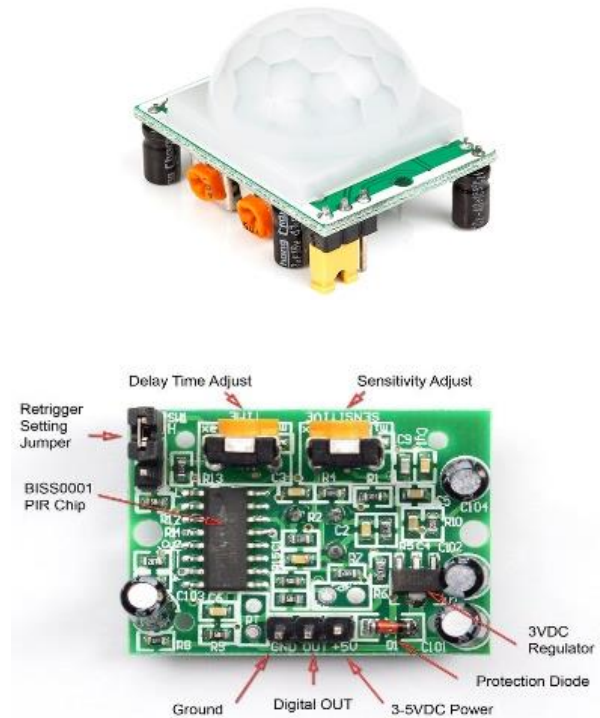
Fig. 7: Passive Infrared Sensor.
