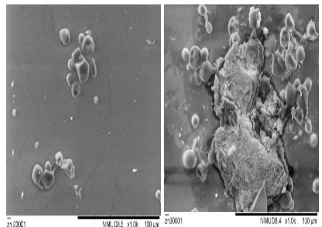
Fig. 3: FESEM micrograph of a) 3 mg/ml and b) 5 mg/ml of zinc oxide nanoparticle with glutinous flour solution coated on mango
