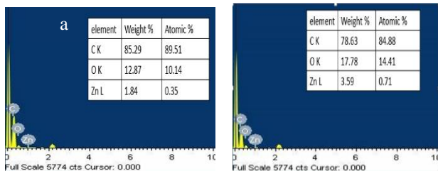
Fig. 4: EDX analysis of (a) control mango, (b) 3 mg/ml ZnO nanoparticles with glutinous flour solution and (c) 5 mg/ml ZnO nanoparticles with glutinous flour solution
