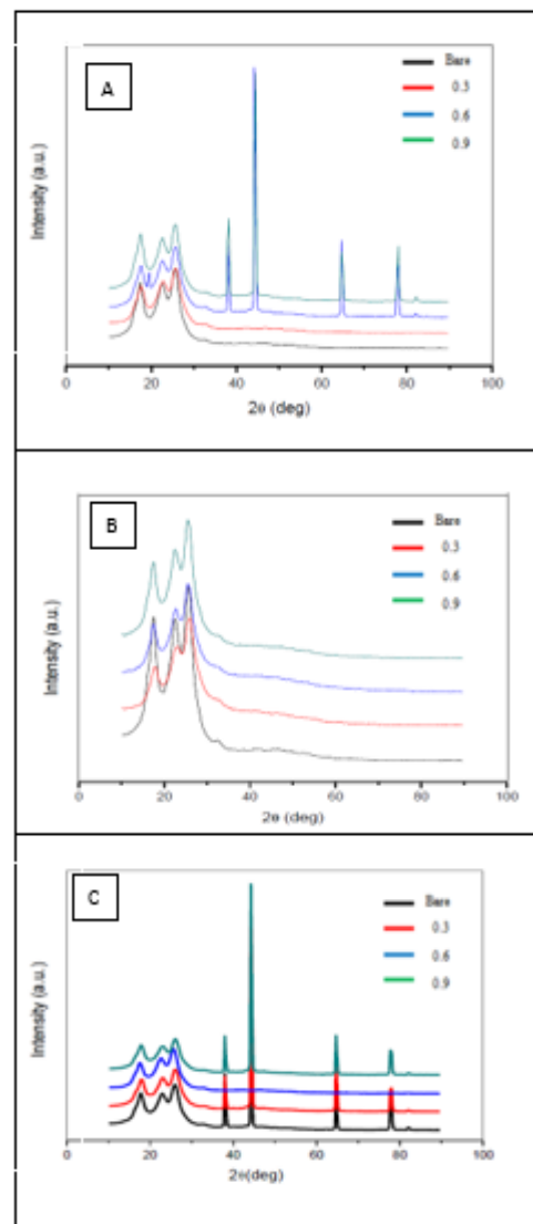
Fig. 3: X-Ray diffractogram of A) undoped PANI-EB B) doped PANI with sulphuric acid C) doped PANI with p TSA
