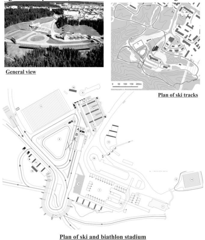
Fig. 4. Winter Sports Center in Khanty-Mansiysk (Russia)
