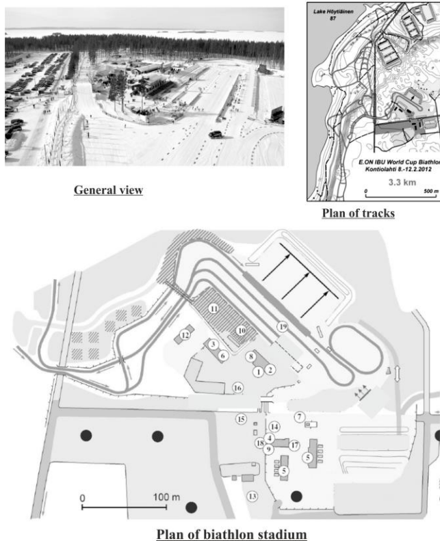
Fig. 2: Biathlon sports club in Kontiolahti (Finland)
