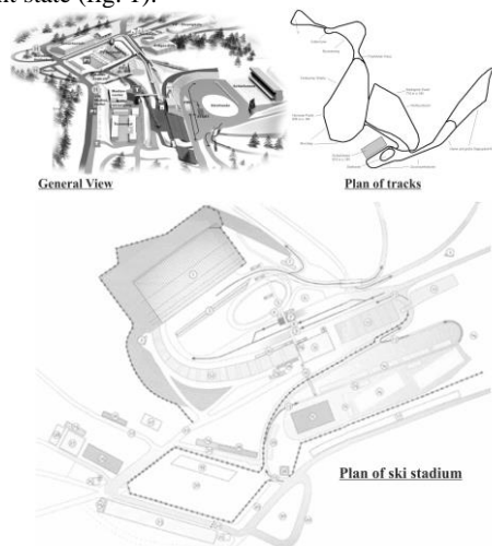
Fig. 1: DKB-Ski-Arena in Oberhof (Germany)
