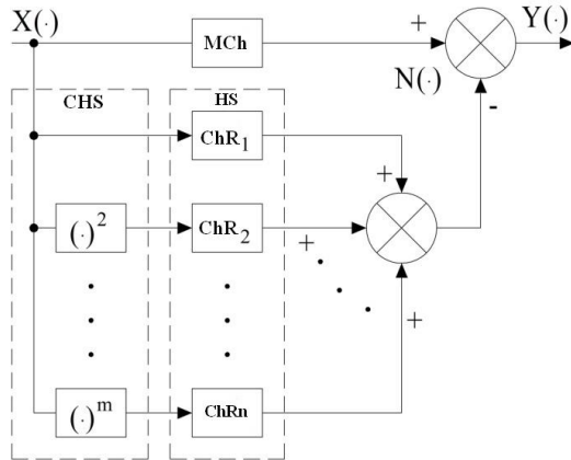
Fig.1: General structural diagram of a one-dimensional adaptive compensator of nonlinear distortion: MCh – main channel; CHS – reference driver; HS - reference scheme; ChRn - n-y the radio reception channel
