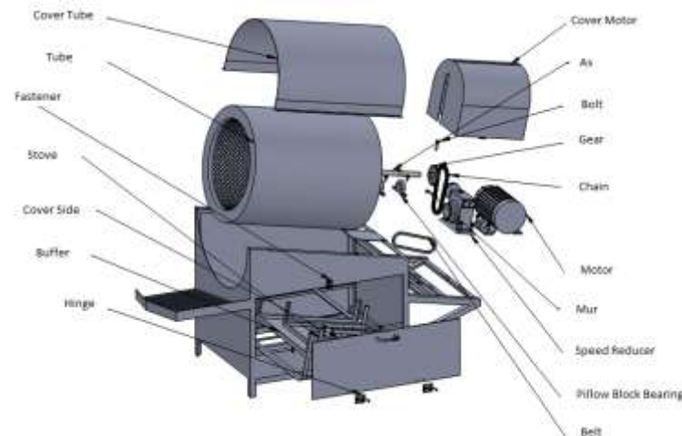
Fig 2: Design Concept Disassembly
