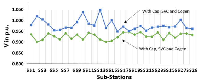
Fig. 9: Network voltage profile before and after the installation of capacitors, SCVs, and cogenerators
