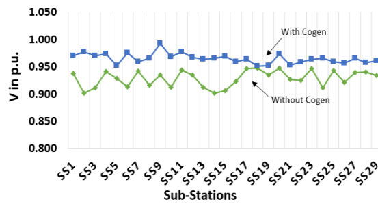
Fig 7: System voltage profile before and after cogenerator installation
