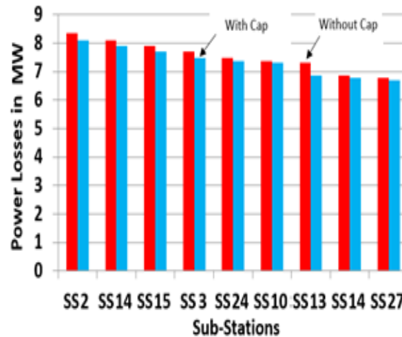
Fig 6: Power losses at the substations before and after capacitor bank installation
