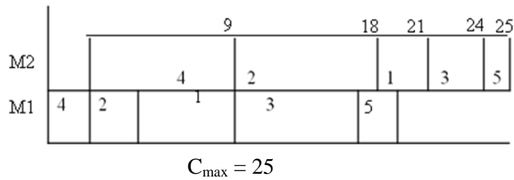
Figure 3: Johnson's algorithm for n = 5, (Optimal schedule T of the jobs)
