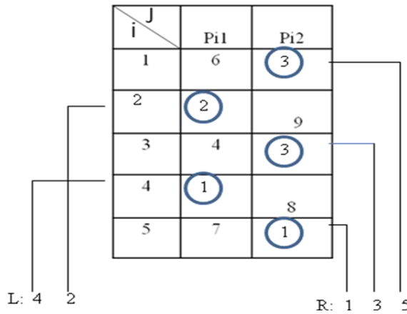
Figure 2: Johnson's algorithm for n = 5 (selecting the jobs)
