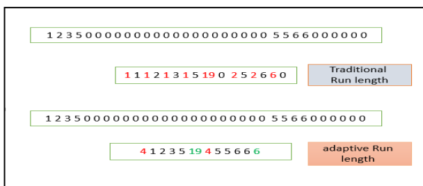
Fig. 8: Difference between Applying an Adaptive RLE and Traditional RLE.
