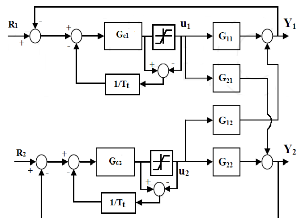
Fig. 1: Decentralized control structure with anti-reset windup
