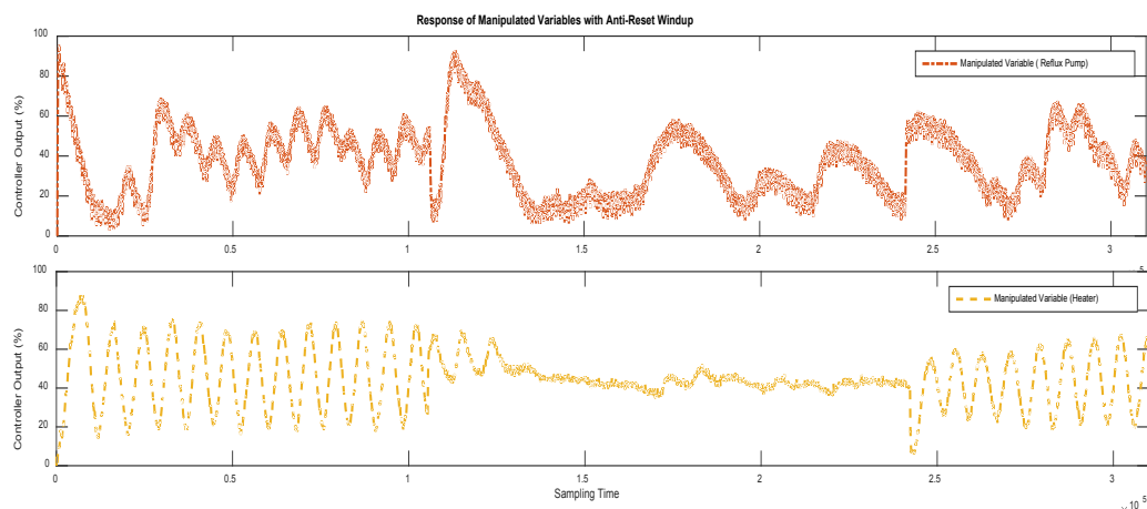
Fig. 11: Controller response with anti-reset windup
