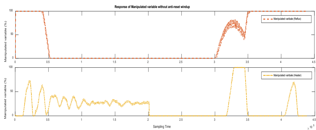
Fig. 9: Controller response without anti-reset windup
