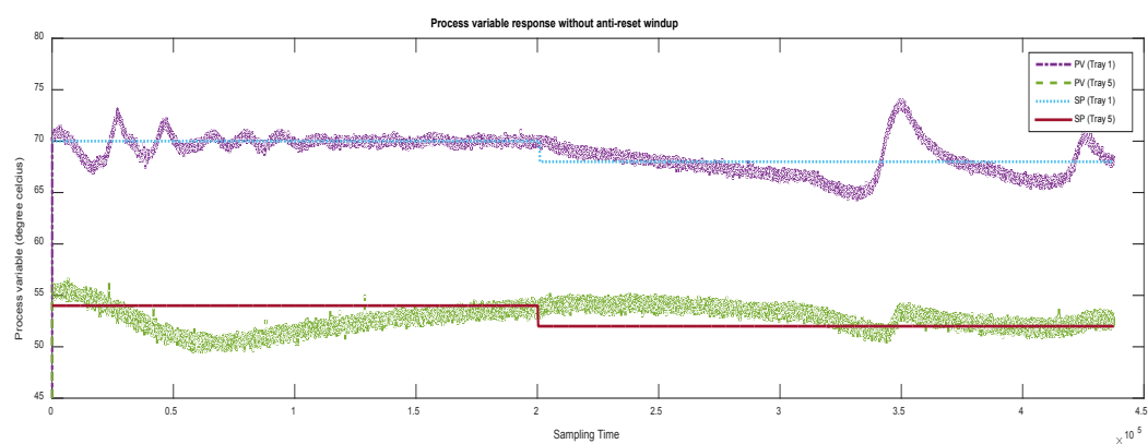
Fig. 8: Closed loop response without anti-reset windup
