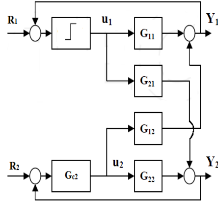
Fig. 4: Relay in loop 1 with loop 2 automated
