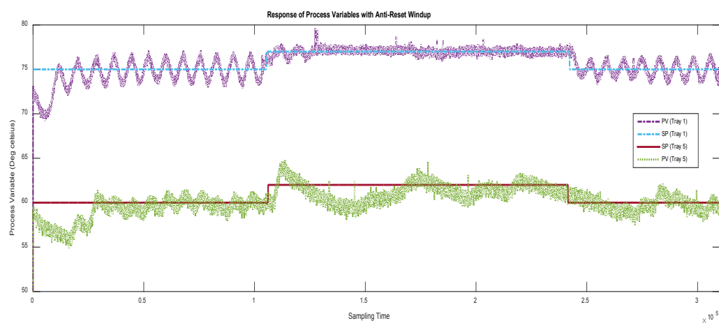
Fig. 10: Closed loop response with anti-reset windup
