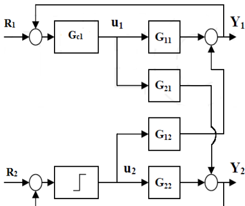
Fig. 3: Relay in loop 2 with loop 1 automated
