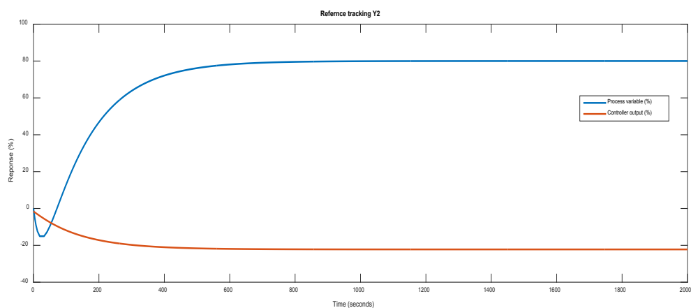
Fig. 7: Closed loop control response of Y_2
