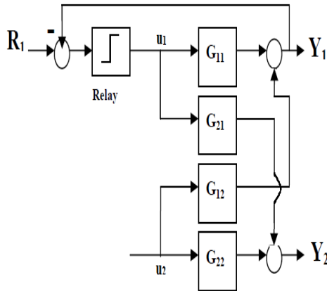
Fig. 2: Ideal relay in loop 1
