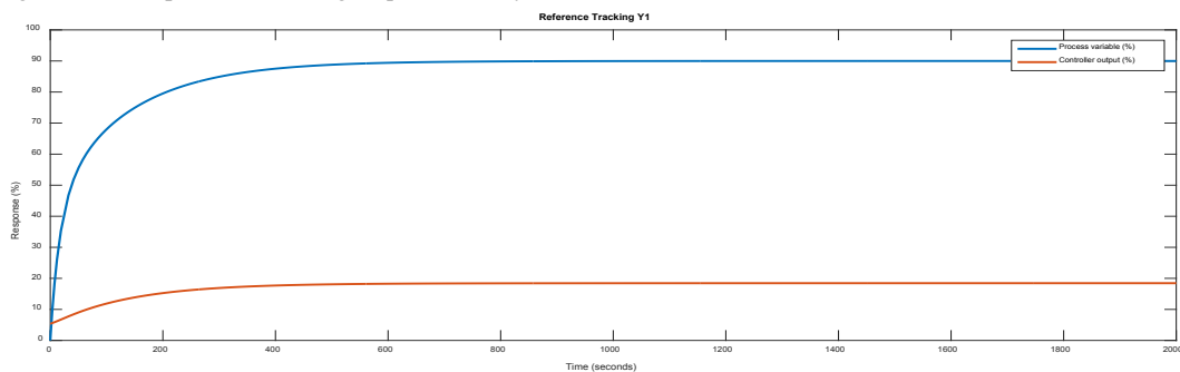
Fig. 6: Closed loop control response of Y 1
