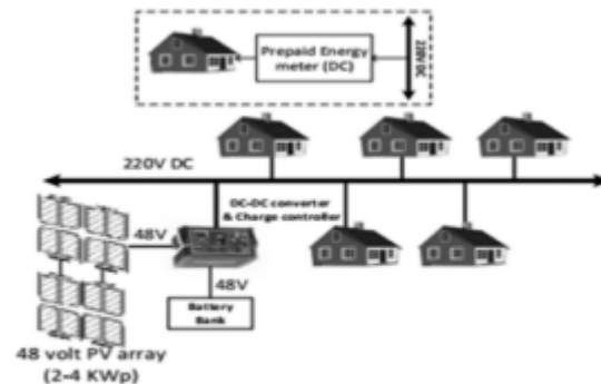
Figure 1: Model of a Typical Nanogrid
