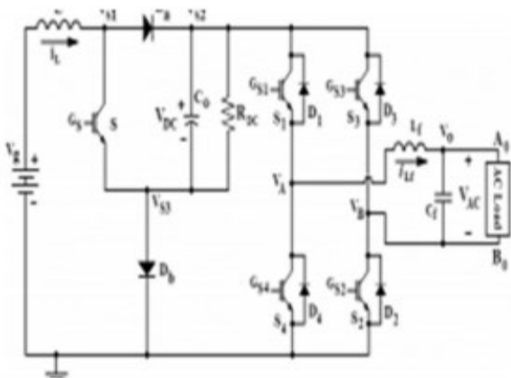
Figure 2 : Circuit of CFSI
