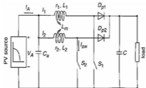
Figure 4: Interleaved Buck Converter
