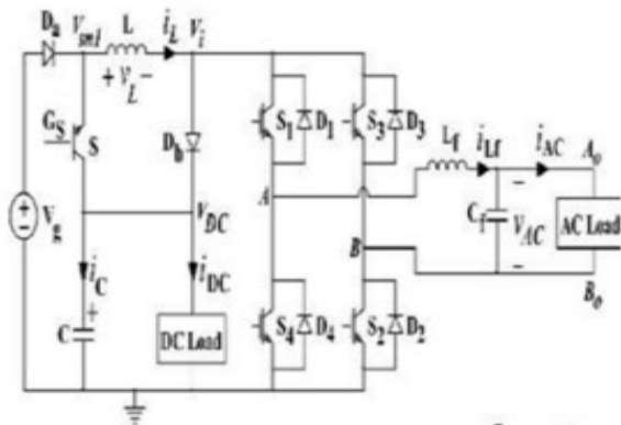
Figure 3 : Circuit of SBI
