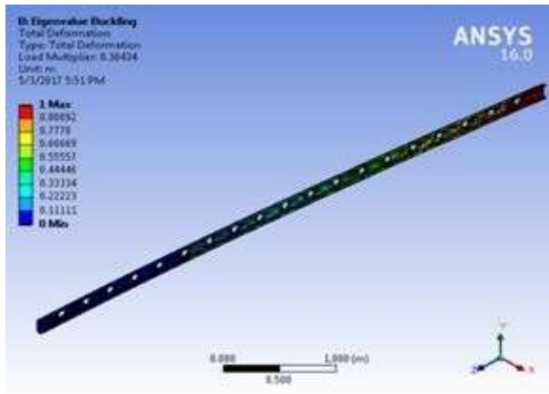
Fig. 8: Total Deflection of C-Section with Type (2) Circular Opening.
