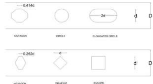
Fig. 4: Geometric Configuration of Perforation. D is the Width of per Foration.
