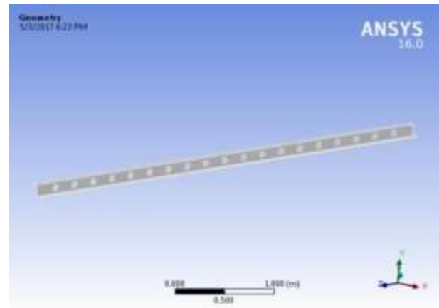
Fig. 10: ANSYS Model of Z Section with Type (2) Circular Perforation.
