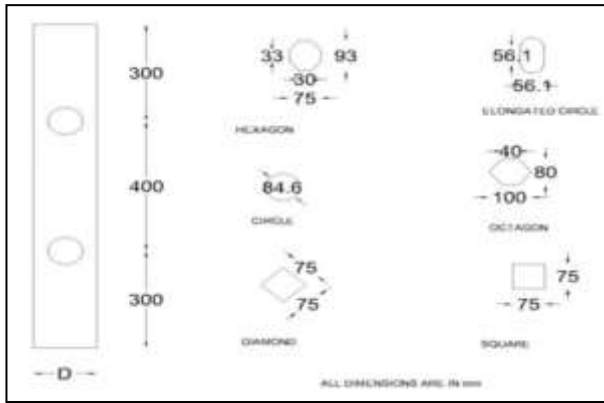
Fig. 5: Dimensions of Perforations with Equal Area.
