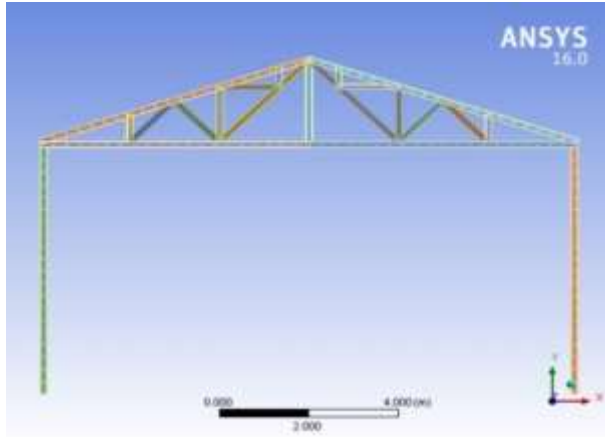
Fig. 12: ANSYS Model of Frame with Type (1) Perforation.
