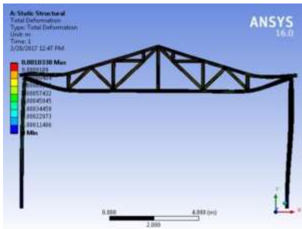
Fig. 13: Total Deformation of Frame with Type (1) Perforation.
