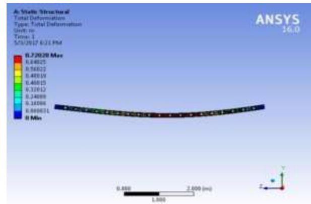
Fig. 11: Total Deflection of Z Section with Type (2) Circular Opening.
