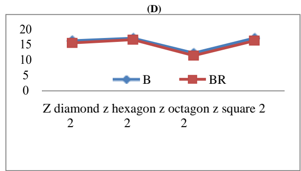
Fig. 9: Percentage Reduction in Buckling Load Due to Corner Rounding For Various Shapes of Perforations (A) C Section with Type 1 Perforation B) Z with Type 1 C) C with Type 2 D) Z With Type 2 ( Percentage in Y-Axis).
