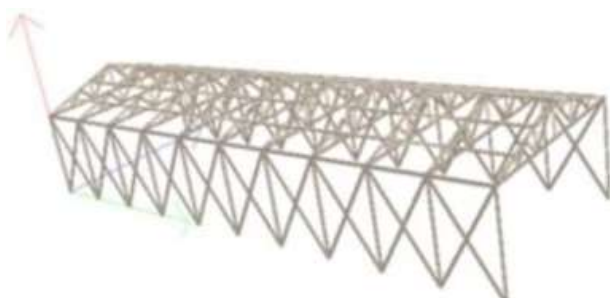
Fig. 3: Rendered View of the STAAD Pro Model of Selected Trussed Building.
