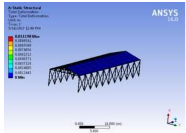
Fig. 15: Total Deformation of Building with Type (1) Perforation.
