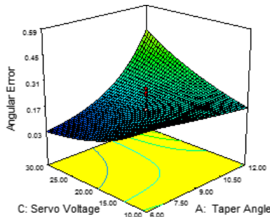
Fig. 6: Surface Plots Showing Effect of Servo Voltage and Taper Angle on Angular Error.
