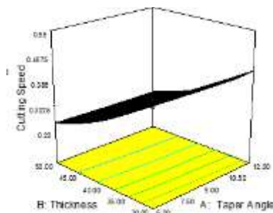
Fig. 1: Surface Plots Showing Effect of Taper Angle and Thickness on Cutting Speed.
