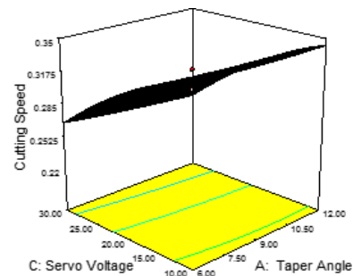
Fig. 3: Surface Plots Showing Effect of Servo Voltage and Taper Angle on Cutting Speed.
