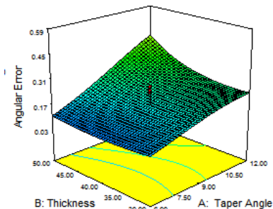
Fig. 4: Surface Plots Showing Effect of Taper Angle and Thickness on Angular Error.
