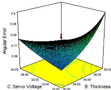
Fig. 5: Surface Plots Showing Effect of Servo Voltage and Thickness on Angular Error.
