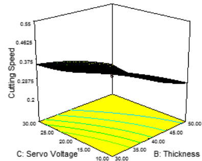
Fig. 2: Surface Plots Showing Effect of Servo Voltage and Thickness on Cutting Speed.
