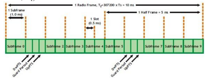
Fig. 3: Type 2 Body Type. Special Fields are Shown of Sub-Frames 1 and 6. Guard Duration Separates the Downlink and Uplink. This TDD Example Represents A 5ms Swap Point. A 10ms Swap Factor Would Now Not Bear the Distinct Fields in Sub-Frame 6.
