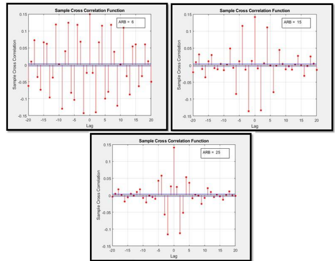
Fig. 12: Cross Correlation Test of LTE Uplink Waveform between 16 QAM and QPSK Modulation Using Various ARB.
