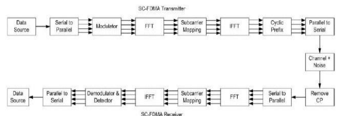
Fig. 4: SC-FDMA System. Block Diagram.
