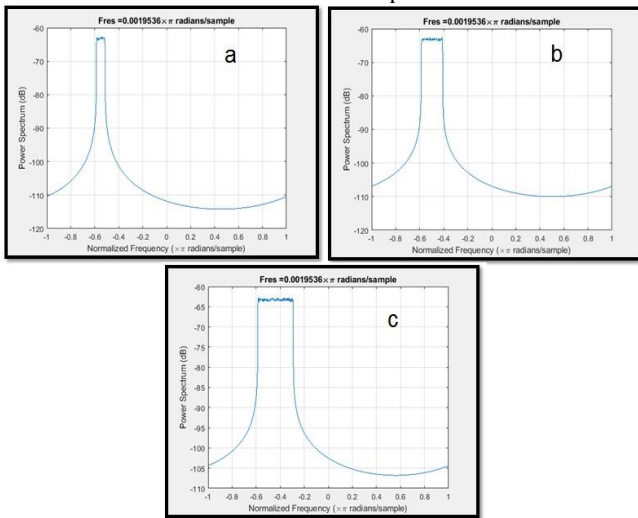
Fig. 5: LTE Uplink RMC Wave Form with QPSK Modulation and FDD Duplex Mode, A- RB 6, B- RB 15, C- RB 25.
