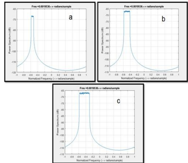
Fig. 7: LTE Uplink RMC Wave Form with QPSK Modulation and TDD Duplex Mode, A- RB 6, B- RB 15, C- RB 25.
