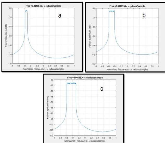
Fig. 6: LTE Uplink RMC Wave Form with 16 QAM Modulations and FDD Duplex Mode, A- RB 6, B- RB 15, C- RB 25.
