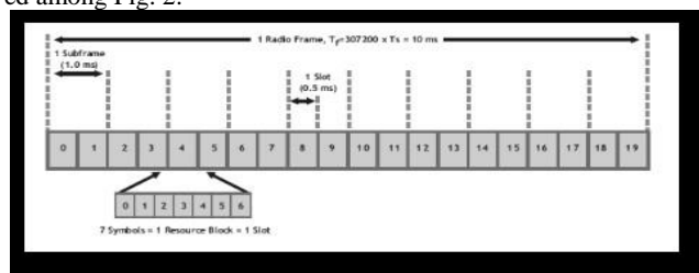
Fig. 2: The Type1 Frame Type. Timing & Symbol Allocations Proven For FDD with Normal Cyclic Prefix.
