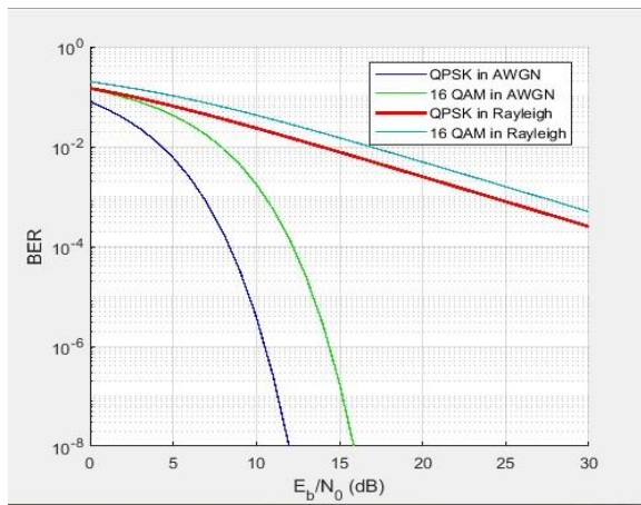
Fig. 9: QPSK And 16 QAM under AWGN and Rayleigh Fading Channel.
