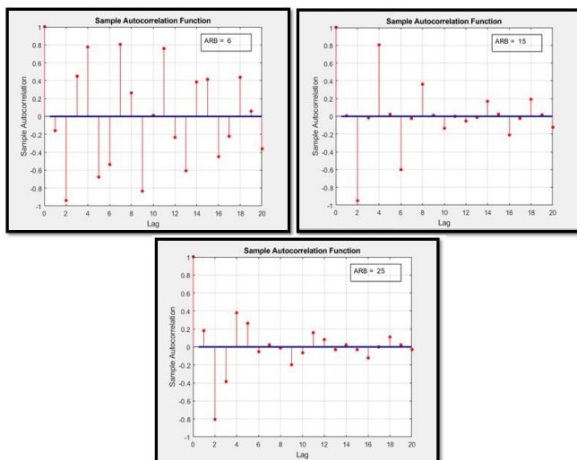
Fig. 11: Autocorrelation Test of LTE Uplink Waveform with 16 QAM Modulations Using Various ARB.
