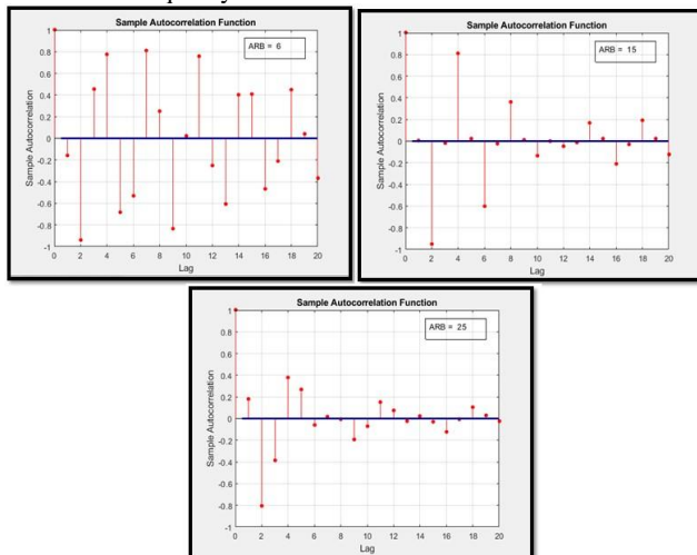
Fig. 10: Autocorrelation Test of LTE Uplink Waveform with QPSK Modulation Using Various Allocated Resources Blocks AEB.
