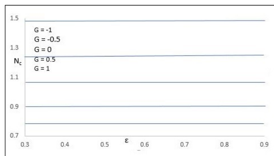
Fig. 4: The variation of N_c versus \varepsilon for various estimations of G
