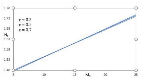
Fig. 2: Variation of N_c versus M_3 for various estimations of \varepsilon
