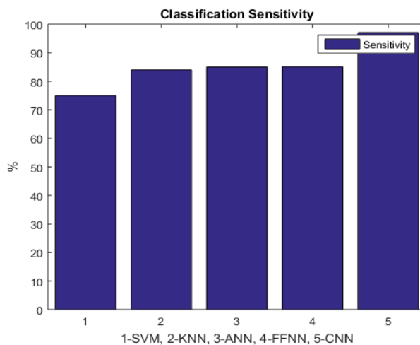
Fig. 6: Performance Analysis of Sensitivity.
