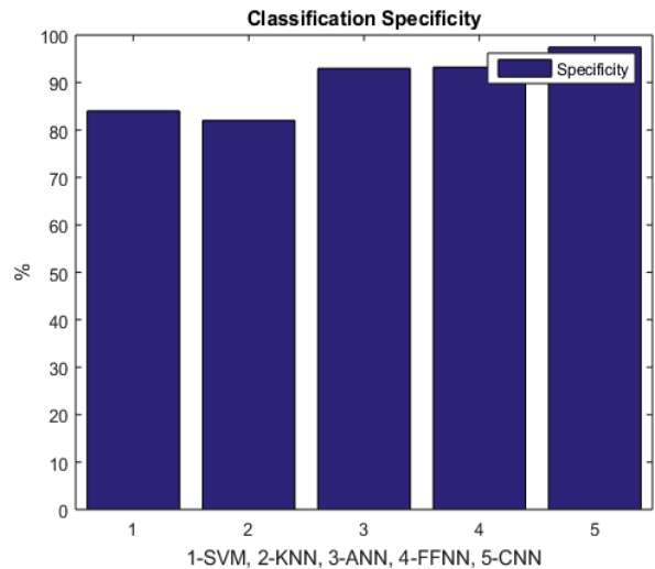
Fig. 5: Performance Analysis of Specificity.
