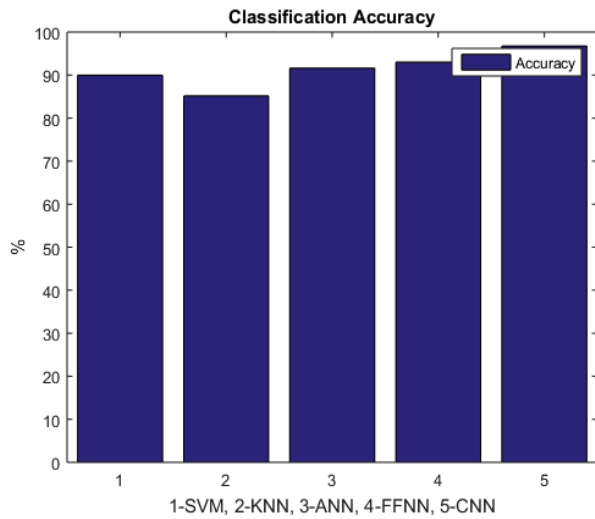
Fig. 4: Performance of Classification Accuracy.
