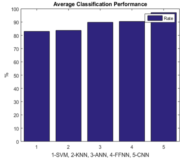
Fig. 7: Average Recognition Rate Performances.
