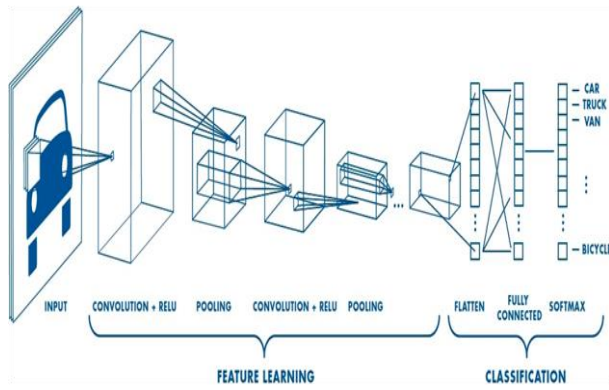
Fig. 3: Working of CNN with Many Convolutional Layers [25].
