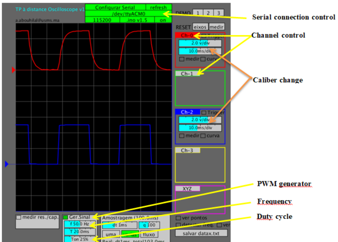
Fig. 3: Developed software oscilloscope-GBF
