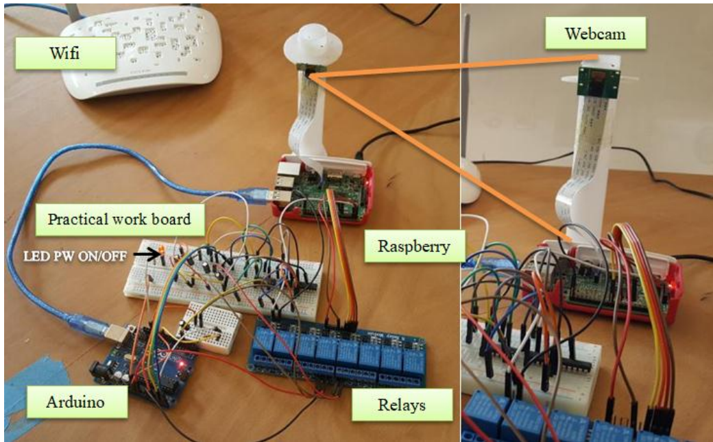
Fig. 4: Realized hardware manipulation
