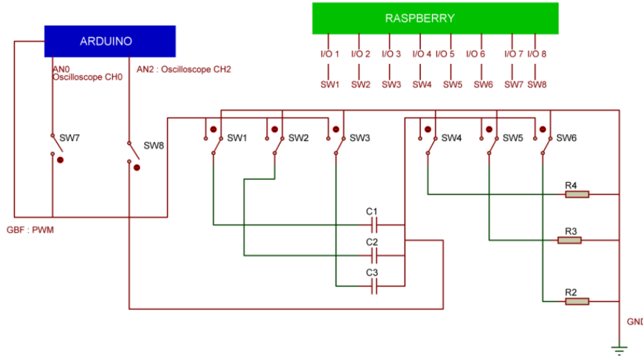
Fig. 2: Web practical work connections
