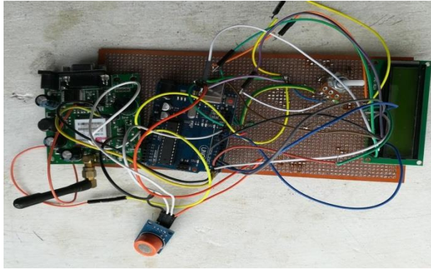
Fig. 2: Real Time Implementation.
