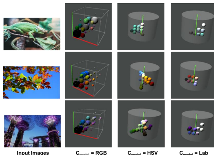
Figure 5: 3D visualization of color distribution according to C_{model}
