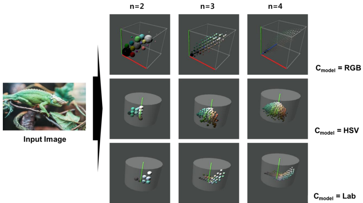
Figure 6: 3D visualization of the color distribution according to C_{model} and n
