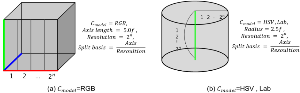
Figure 4: 3D space division model based on color models
