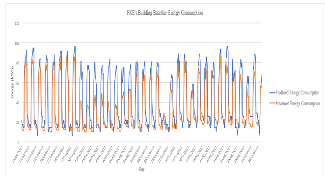
Fig. 4: Multiple Regression Model Energy Prediction FKE's Building
