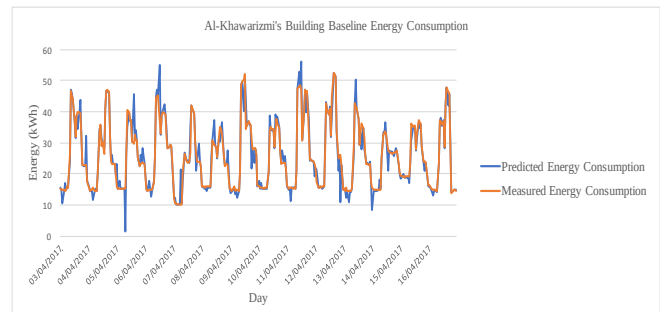
Fig. 9: NARX-ANN Model Energy Prediction Al-Khwarizmi's Building
