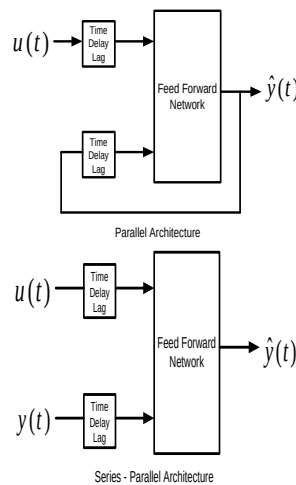
Fig. 2: NARX Model architecture
