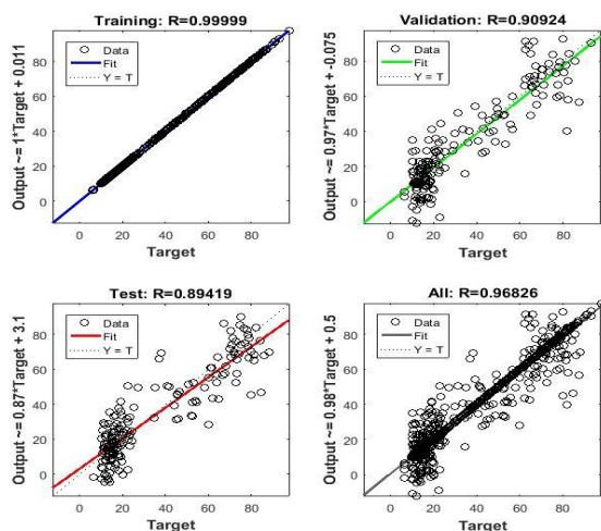
Fig. 6: NARX-ANN Model FKE's Building Regression Plot
