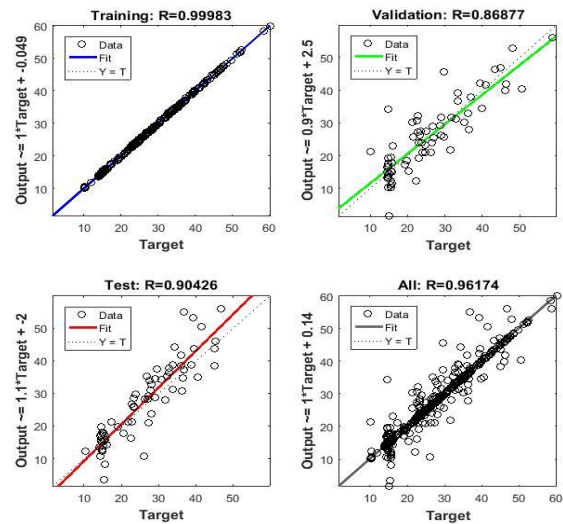
Fig. 7: NARX-ANN Model Al-Khwarizmi's Building Regression Plot.
