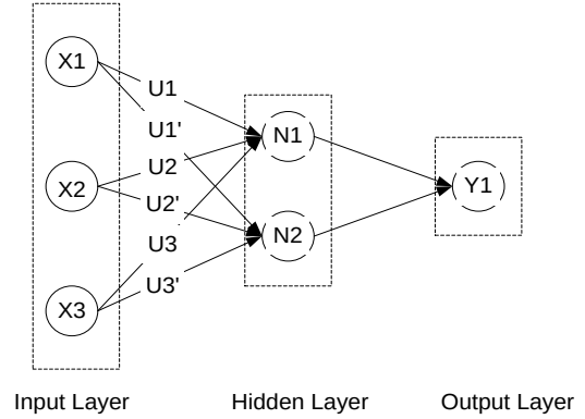
Fig. 1: Multilayer Perceptron Artificial Neural Network
