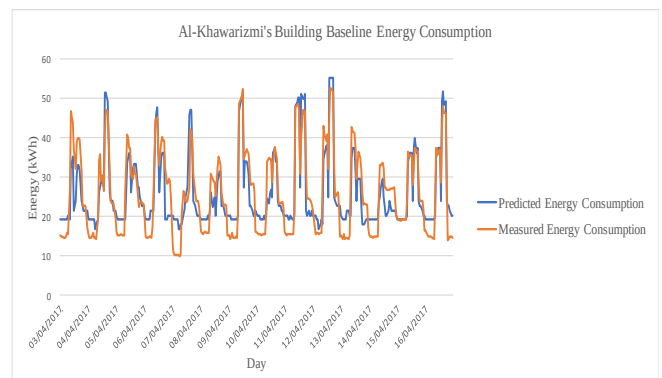
Fig. 5: Multiple Regression Model Energy Prediction Al-Khawarizmi's Building
