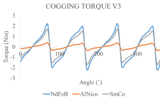
Fig.6: Cogging torque for design V3 with variations of permanent magnet material
