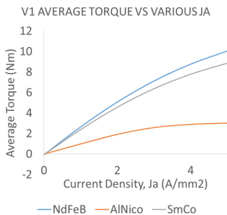
Fig.7: Torque vs various J_A for motor V1 with different permanent magnet material.
