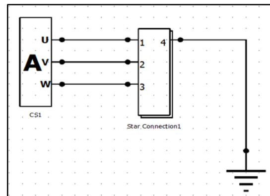
Fig.2: Circuit design for FEM coils
