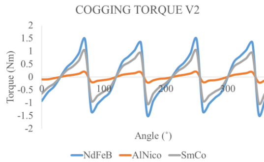
Fig.5: Cogging torque for design V2 with variations of permanent magnet material
