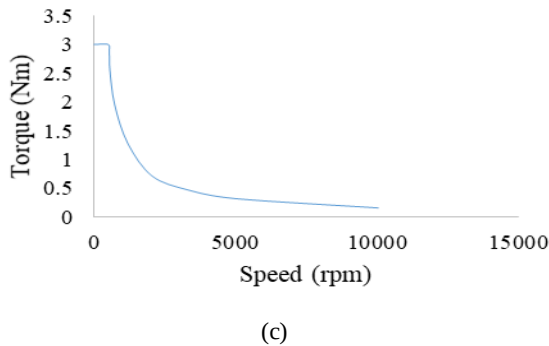
Fig.12: Torque vs speed for motor V3 with different permanent magnet material; (a) NdFeB, (b) AlNiCo, (c), SmCo.
