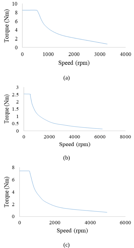
Fig.11: Torque vs speed for motor V2 with different permanent magnet material; (a) NdFeB, (b) AlNiCo and (c), SmCo.
