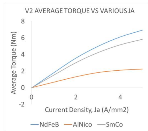
Fig.8: Torque vs various J_A for motor V2 with different permanent magnet material.
