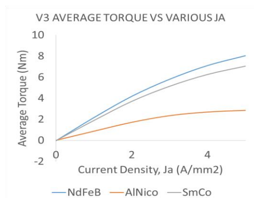
Fig.9: Torque vs various J_A for motor V3 with different permanent magnet material.
