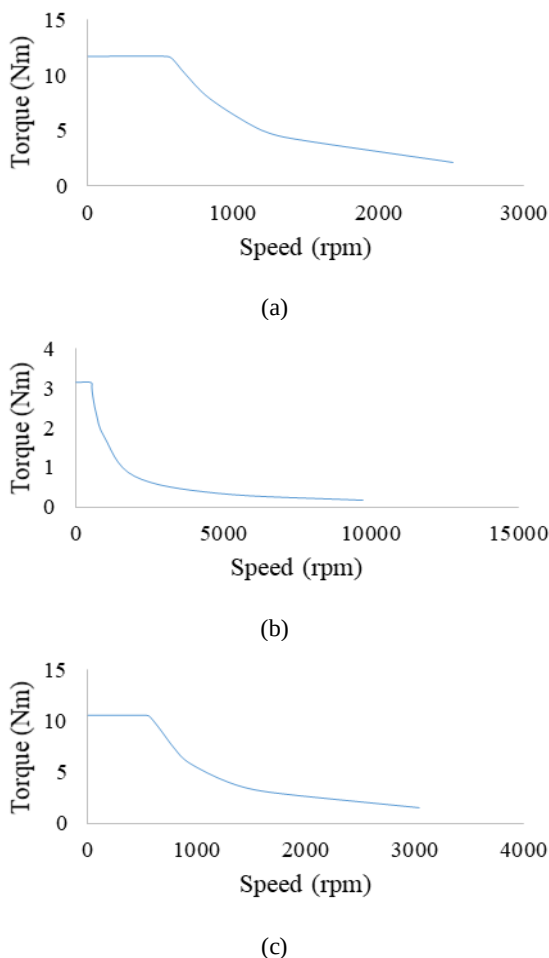
Fig.10: Torque vs speed for motor V1 with different permanent magnet material; (a) NdFeB, (b) AlNiCo, (c) SmCo
