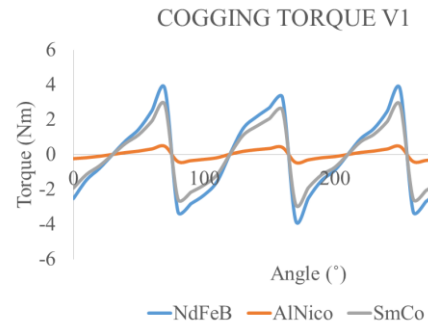
Fig.4: Cogging Torque for design V1 with variation of permanent magnet material
