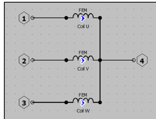
Fig.3: Circuit for FEM coils in Subsystem “Star Connection 1”
