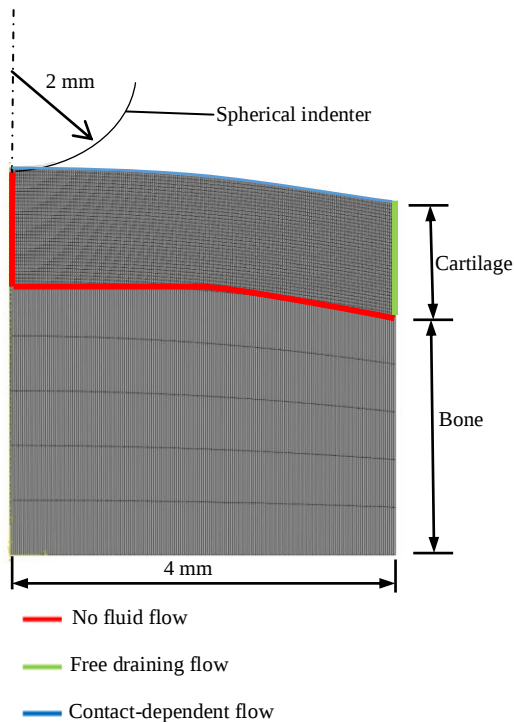
Fig. 4: Axisymmetric FE model of the cartilage specimen.
