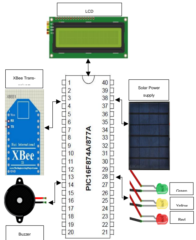
Fig. 9: Traffic Light On-Board Unite Components.
