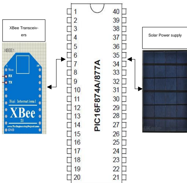
Fig. 10: Vehicle On-Board Unite Components.
