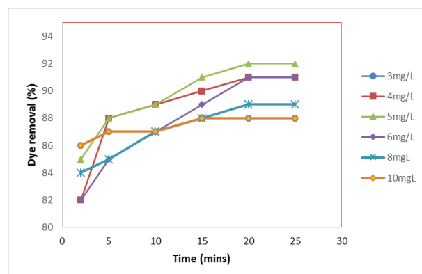
Fig. 3: Time/Concentration Effect of Methylene Blue Adsorption onto Date Palm Leaves Powder at Room Temperature ( 25 \pm 0.5^\circ\text{C} ), Dosage 0.20 G, Ph = 6.0 and Stirring Speed = 1300 Rpm.
