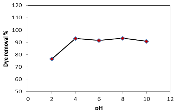
Fig. 4: PH Effect of Methylene Blue Adsorption onto Date Palm Leaf Fibers at Room Temperature ( 25 \pm 0.5 °C), Adsorption Dosage = 200 Mg, Time = 20 Min, Initial Dye Concentration = 4 Mg/L and Stirring Speed = 1300 Rpm.
