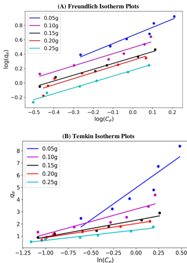
Fig. 5: Freundlich and Temkin Isotherm Plots for the Adsorption of Methylene Blue onto Date Palm Leaf Fibers at Different Adsorbent Dosage.
