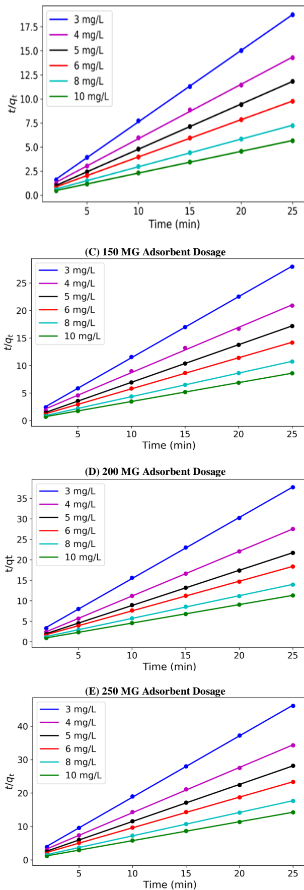
Fig. 6: Pseudo-Second Order Kinetics Plot for the Adsorption of Methylene Blue onto Date Palm Leaf Fibers at Different Adsorbent Dosage.
