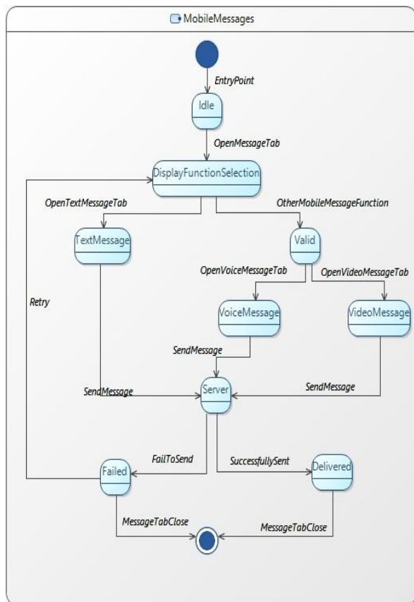
Fig 1: Statechart for sending message by using mobile phone
