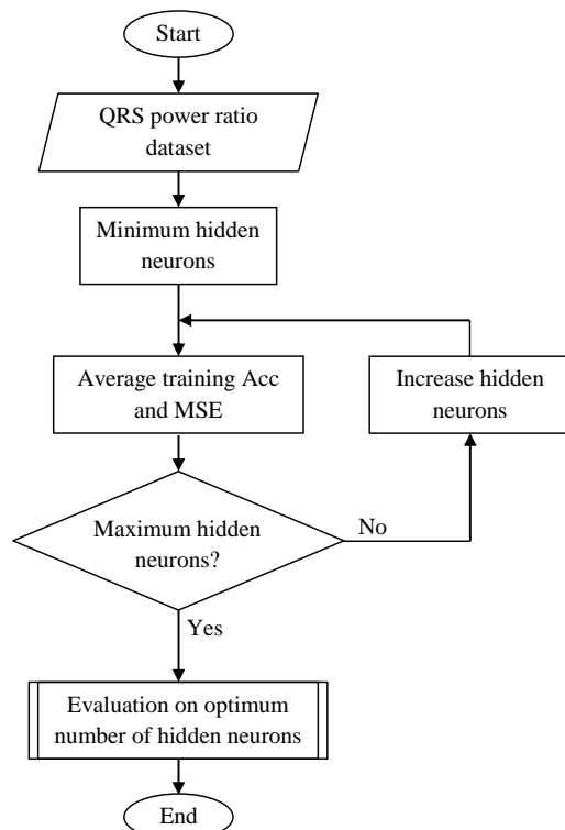
Fig. 2: Exhaustive search algorithm. MSE = Mean Squared Error.
