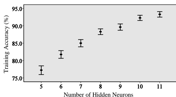
Fig. 3: Average training accuracy.
