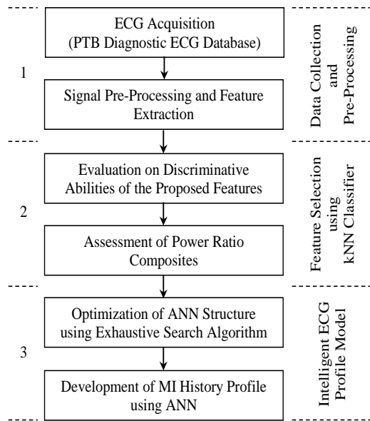
Fig. 1: General framework of research methods.
