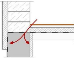
Fig. 2: Increase of the thermal insulation of the wall.
