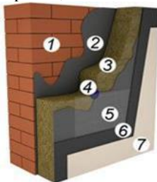
Fig. 4: Wall warming: 1 wall, 2 adhesive layer, 3 insulation, 4 plate dowel 5 reinforcing glass netting, 6 adhesive layer, 7 decorative protective layer.
