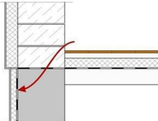
Fig. 3: The thermal insulation of the wall is carried out at 1 m below the ground level.
