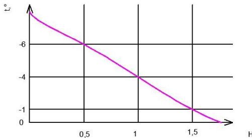
Fig. 1: Graph showing the dependence of the foundation depth on the temperature.
