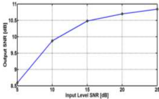
Fig. 4: Relation between input level SNR [dB] and output SNR [dB]
