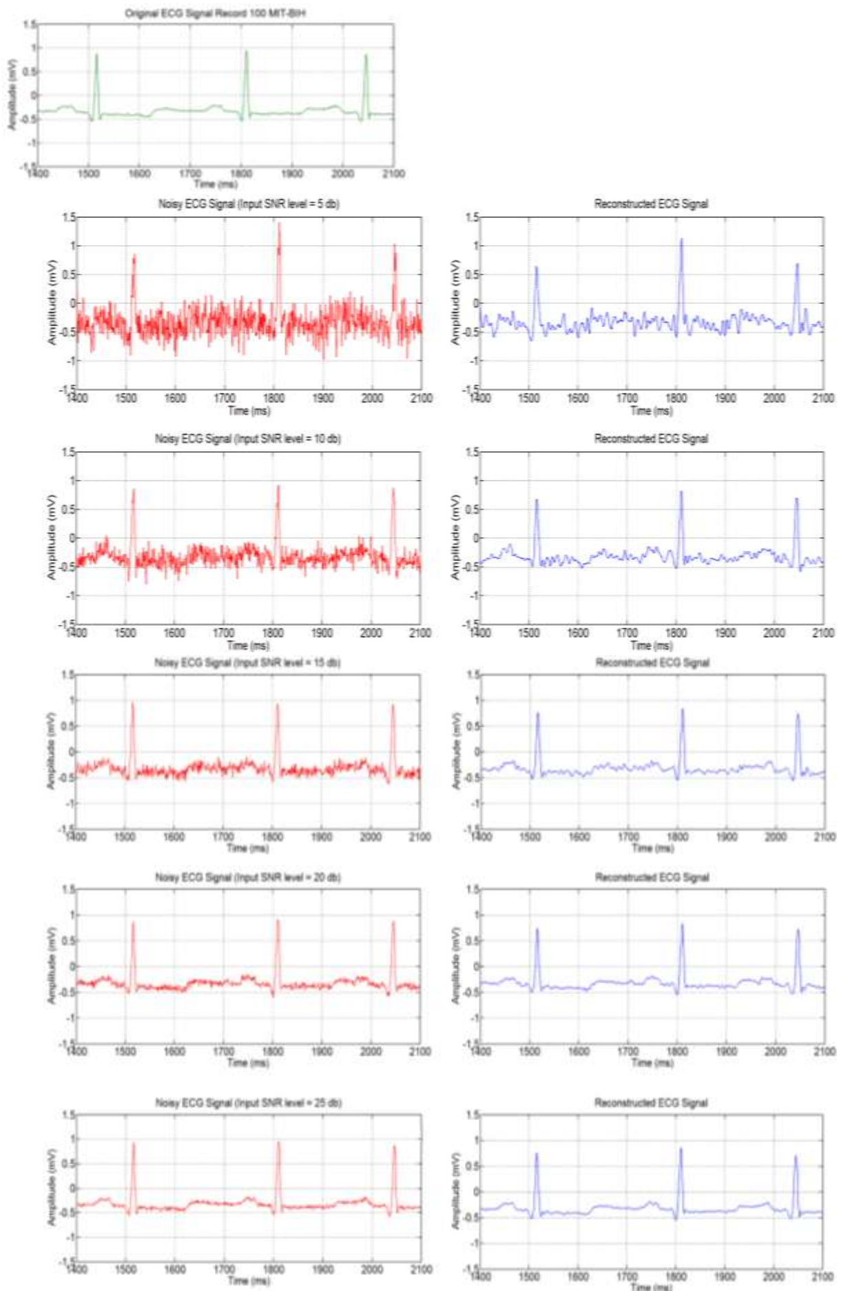
Fig. 3: Original ECG signal record 100 from MIT-BIH DB. In left side, the signal is corrupted with different noise levels (5, 10, 15, 20, and 25 dB) and right side contains the clean signal obtained by proposed approach
