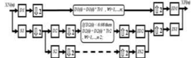
Fig. 2: General block diagram for the proposed approach of ECG signal noise reduction with wavelet hierarchy for 2 levels
