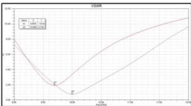
Fig. 5: Simulated VSWR plot of Proposed MIMO PIFA
