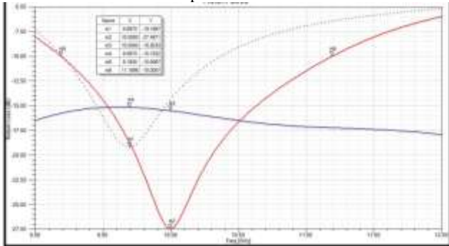
Fig. 3: Simulated Return Loss Plot of Proposed MIMO PIFA
