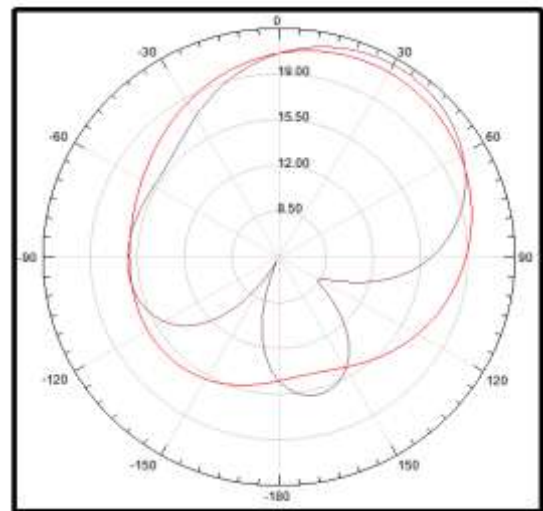
Fig. 7: Simulated Radiation Pattern of Proposed MIMO PIFA
