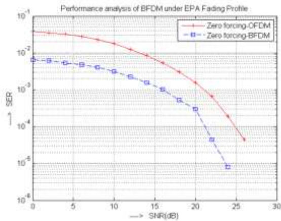
Figure 5: SER analysis of BFDM under EPA fading profile
