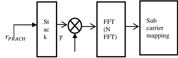
Figure 2: BFDM PRACH receiver
