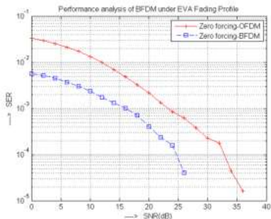
Figure 6: SER analysis of BFDM under EVA fading profile
