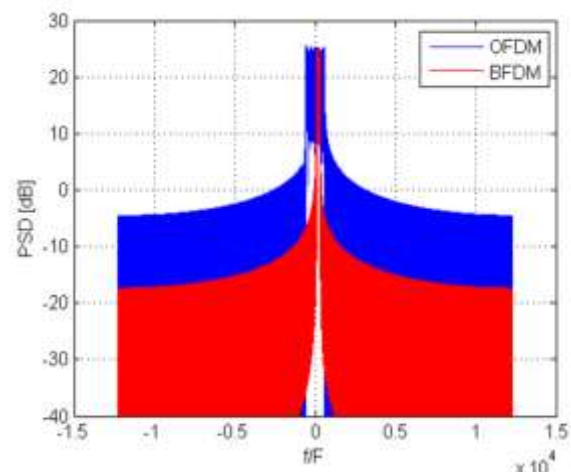
Figure 4: PSD of BFDM and OFDM systems
