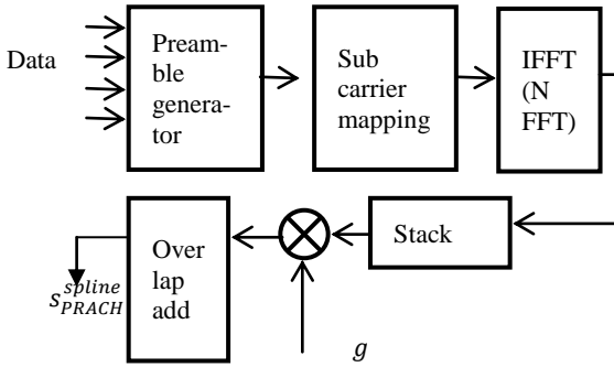
Figure 1: BFDM PRACH transmitter
