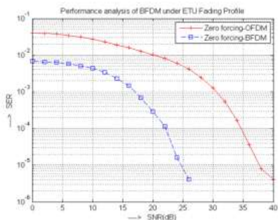
Figure 7: SER analysis of BFDM under ETU fading profile
