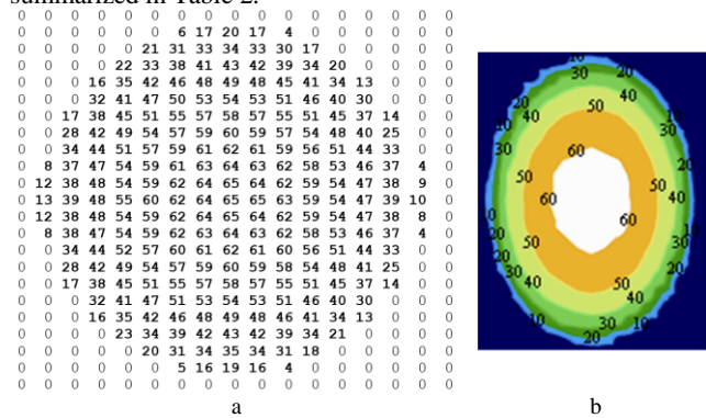
Fig. 6: Distribution of contact pressures, kgf/mm 2 : a - in numerical form (based on the calculation results in the NZD program); b - in a contour form (processing of results of calculations in the program environment MathCad)
