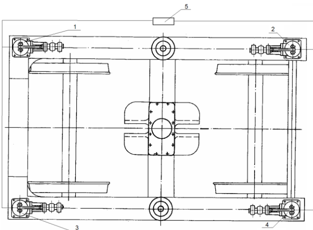
Fig. 8: Scheme of placing the CCS on the locomotive bogie
