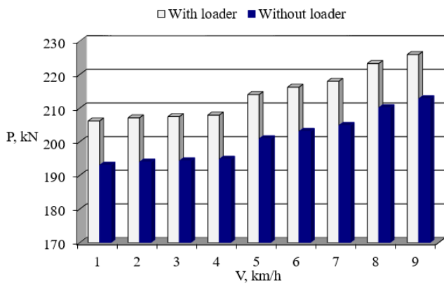
Fig. 5: Dependence of changes in loads Q on the first wheel pair on the speed of movement
