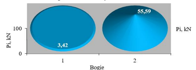
Fig. 7: Difference of vertical loads \Delta P_i along i -th axes of bogies of diesel locomotive TEM103
