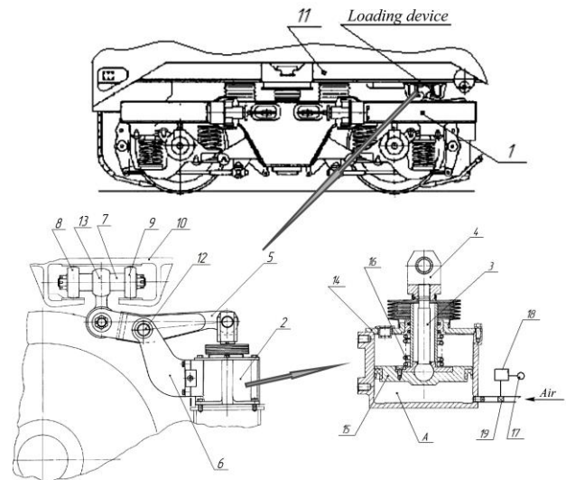
Fig. 1: Scheme of installation of the loading device on the bogie of the shunting locomotive TEM103
