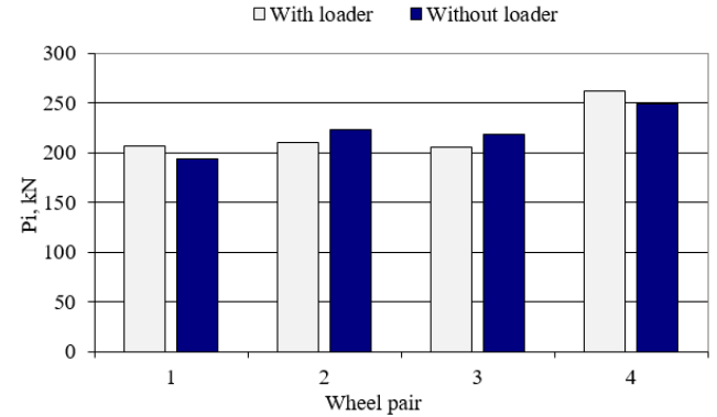
Fig. 3: Efforts in wheel pairs at a speed V = 3 km/h.
