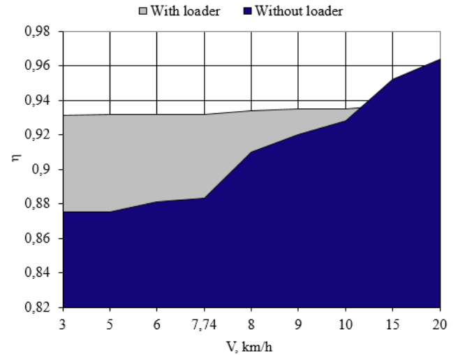
Fig. 4: The change in the coefficient of use of the coupling weight ( \eta ) of the first wheel pairs from the speed ( V )
