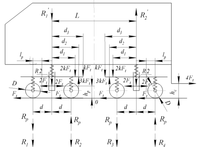
Fig. 2: Diagram of geometric parameters and forces acting on the locomotive.
