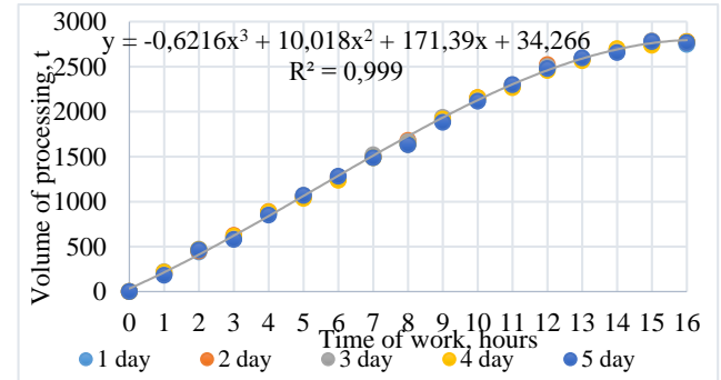
Fig. 2: Checking the model for adequacy for the transport enterprise
