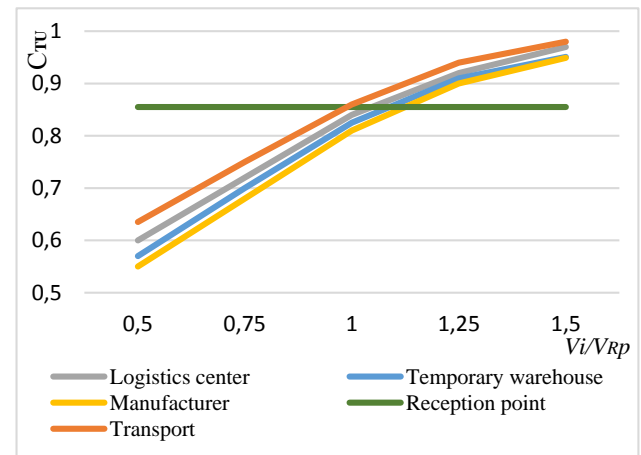
Fig. 3: Dependences of the change of the coefficient technical use of logistic links on the ratio of cargo processing volumes in the supply chain.
