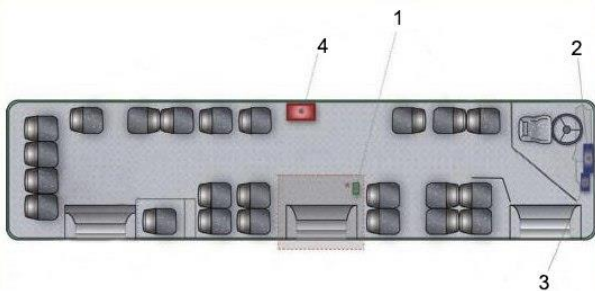
1- equipment for counting entering/leaving passengers; 2- information module; 3- global positioning equipment (GPS); 4- validators;
