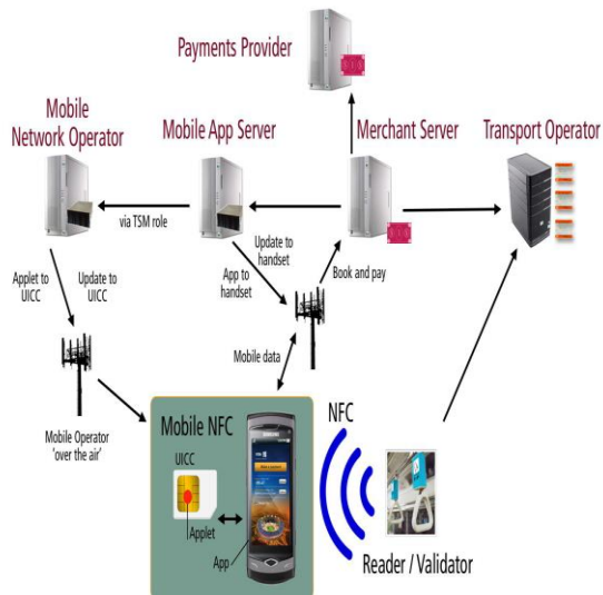
Fig. 3 Using NFC mobile module with UICC card
