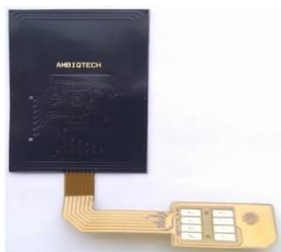
Figure 2 The NFC module sticker
