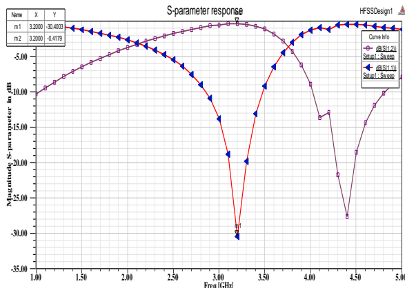
Fig.3: EM simulation result for the proposed bandpass DGS filter
