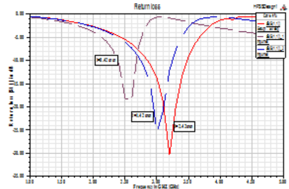
Fig.5: EM simulation of return loss for the different values of the geometrical parameter l
