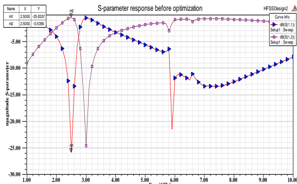
Fig.2: EM simulation result before optimization
