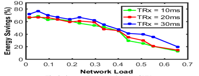
Fig. 8: Average Energy savings per ONU
