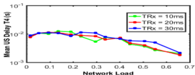
Fig. 14: Mean upstream delay of T4 traffic per ONU
