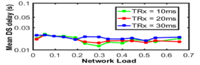
Fig. 9: Mean downstream delay per ONU
