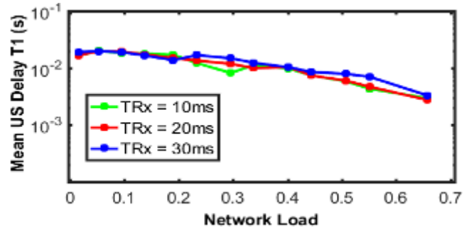
Fig. 11: Mean upstream delay T1 traffic per ONU
