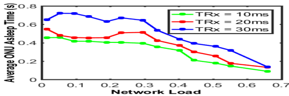
Fig. 5: Average ONU Asleep State time
