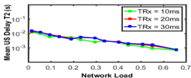
Fig. 12: Mean upstream delay of T2 traffic per ONU
