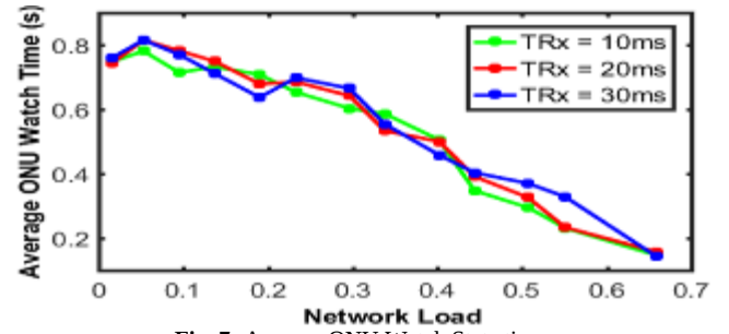
Fig. 7: Average ONU Watch State time
