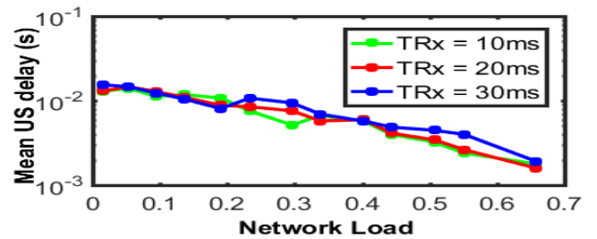
Fig. 10: Overall mean upstream delay per ONU
