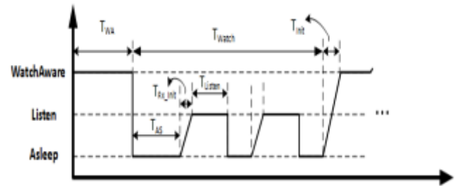
Fig. 4: State transition process of Watchful sleep Mode
