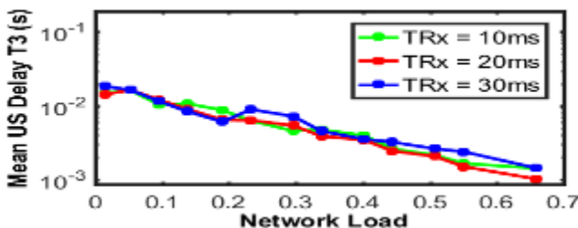
Fig. 13: Mean upstream delay of T3 traffic per ONU
