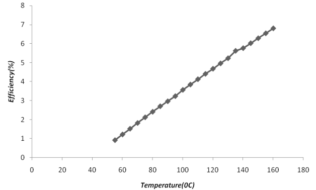
Graph. 5: Efficiency as a Function of Temperature.
