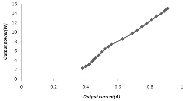
Graph. 1: Output Power as a Function of Output Current.
