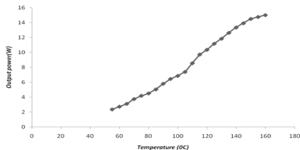
Graph. 4: Output Power as a Function of Temperature.
