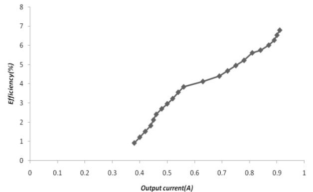
Graph. 6: Efficiency as a Function of Output Current.
