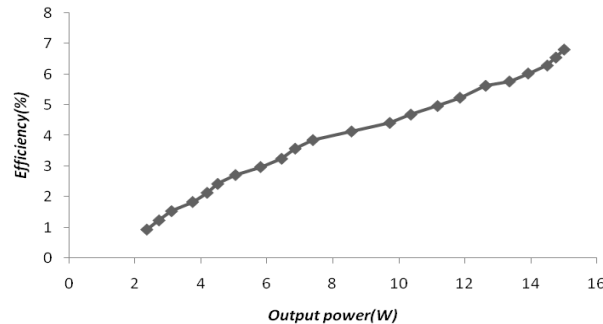
Graph. 2: Efficiency as a Function of Output Power.
