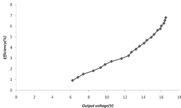
Graph. 3: Efficiency as a Function of Output Voltage.
