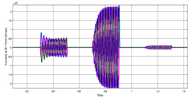
Fig. 9: Current Waveform at B1 Point.
