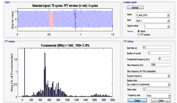
Fig. 16: Harmonic Spectrum of Load Voltage at T = 0.5sec (for Sag Condition).
