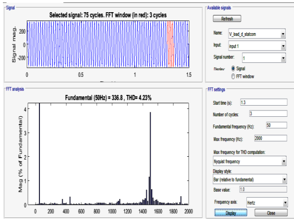
Fig. 25: Harmonic Spectrum of Load Voltage at T = 1.3 Sec (for Harmonics Caused Due to Non-Linear Load).
