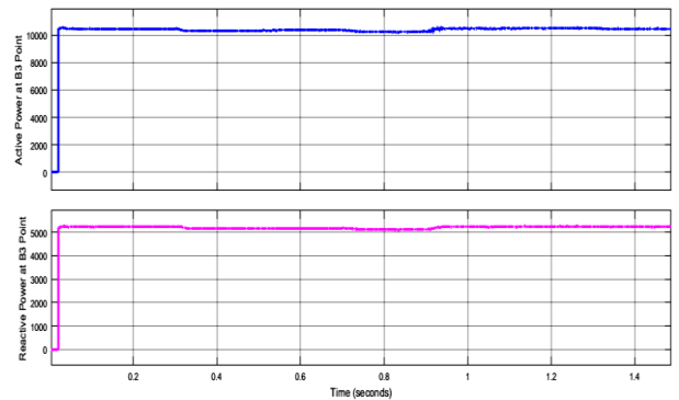
Fig. 22: Active and Reactive Power at B3 Point.
