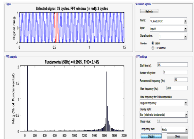
Fig. 30: Harmonic Spectrum of Load Voltage at T = 0.5Sec (for Sag Condition).
