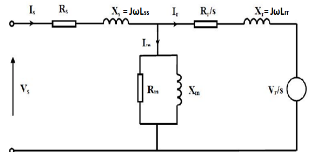
Fig. 3: Equivalent Circuit of DFIG.
