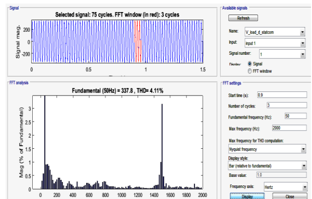
Fig. 24: Harmonic Spectrum of Load Voltage at T = 0.9 sec (for Swell Condition).
