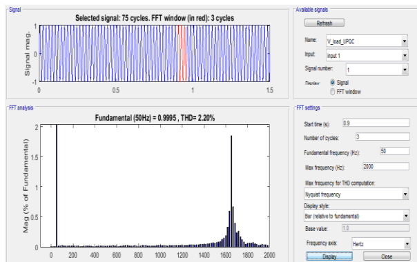
Fig. 31: Harmonic Spectrum of Load Voltage at T = 0.9sec (for Swell Condition).
