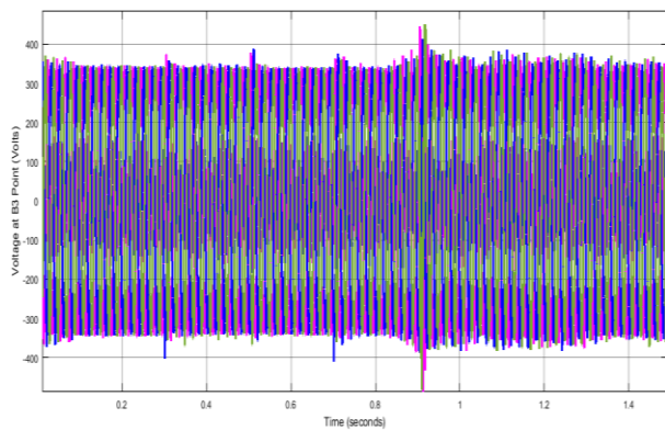
Fig. 13: Voltage Waveform at B3 Point.
