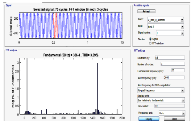
Fig. 23: Harmonic Spectrum of Load Voltage at T = 0.5 Sec (for Sag Condition).
