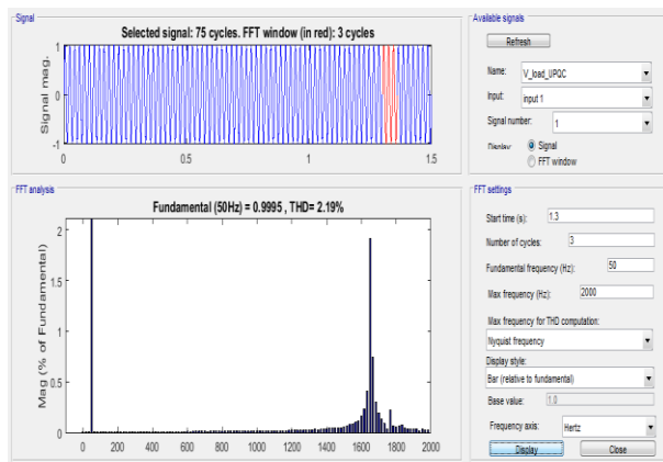
Fig. 32: Harmonic Spectrum of Load Voltage at T = 1.3 Sec (for Harmonics Caused Due to Non-Linear Load).
