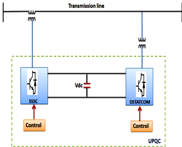
Fig. 6: Schematic Diagram of UPQC.
