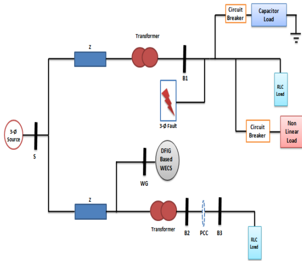
Fig. 1: Single Line Diagram of Study Case Power System.
