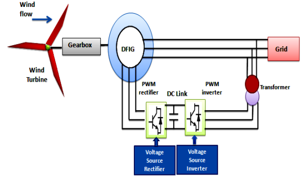
Fig. 2: Wind Energy Conversion System with DFIG.
