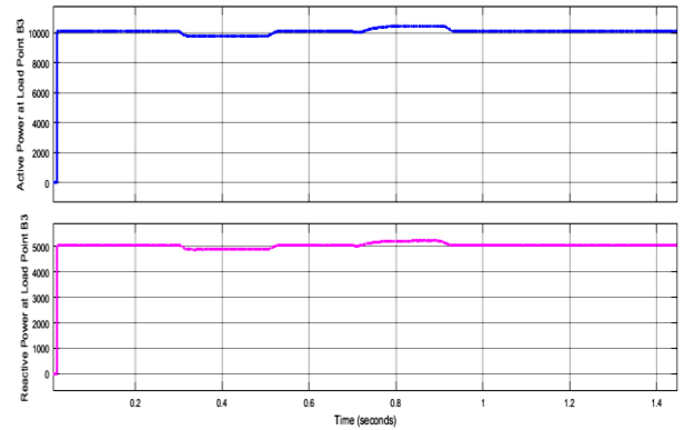
Fig. 15: Active and Reactive Power at B3 Point.
