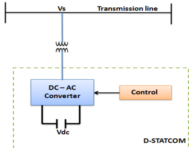
Fig. 5: Schematic Diagram of D-STATCOM.
