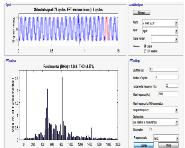
Fig. 18: Harmonic Spectrum of Load Voltage at T = 1.3 Sec (for Harmonics Caused Due to Non-Linear Load).
