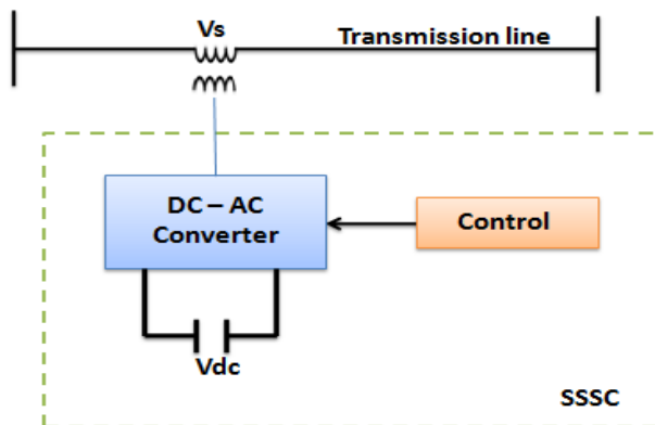
Fig. 4: Schematic Diagram of SSSC.
