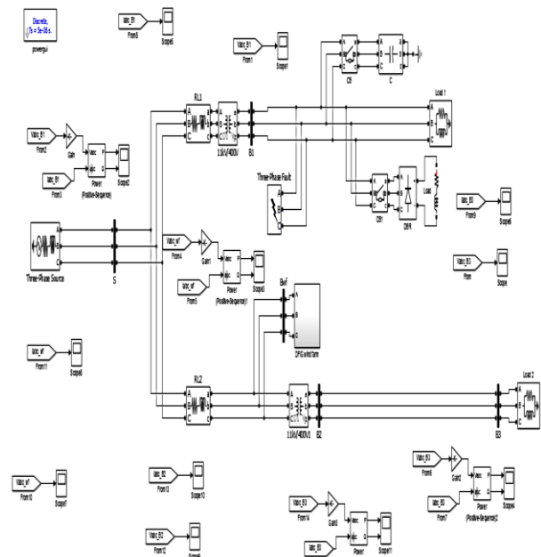
Fig. 7: MATLAB/SIMULINK Model for Test System.
