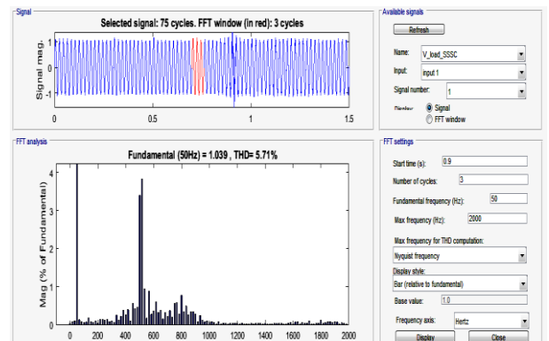
Fig. 17: Harmonic Spectrum of Load Voltage at T = 0.9sec (for Swell Condition).
