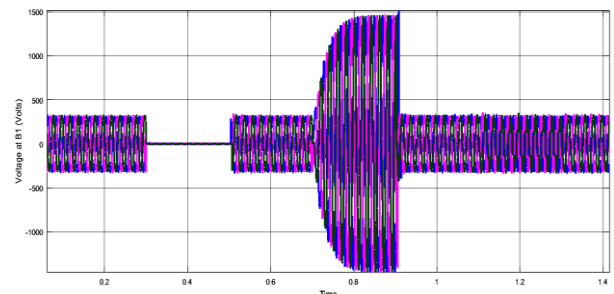
Fig. 8: Voltage Waveform at B1 Point.
