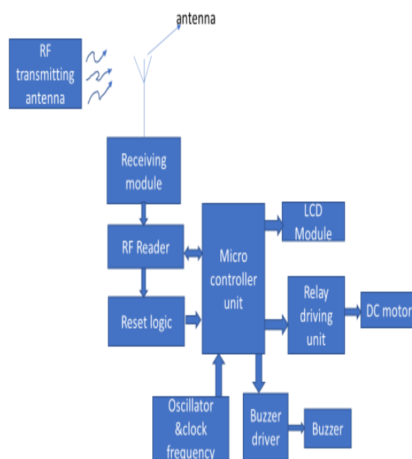
Complete Block Diagram
