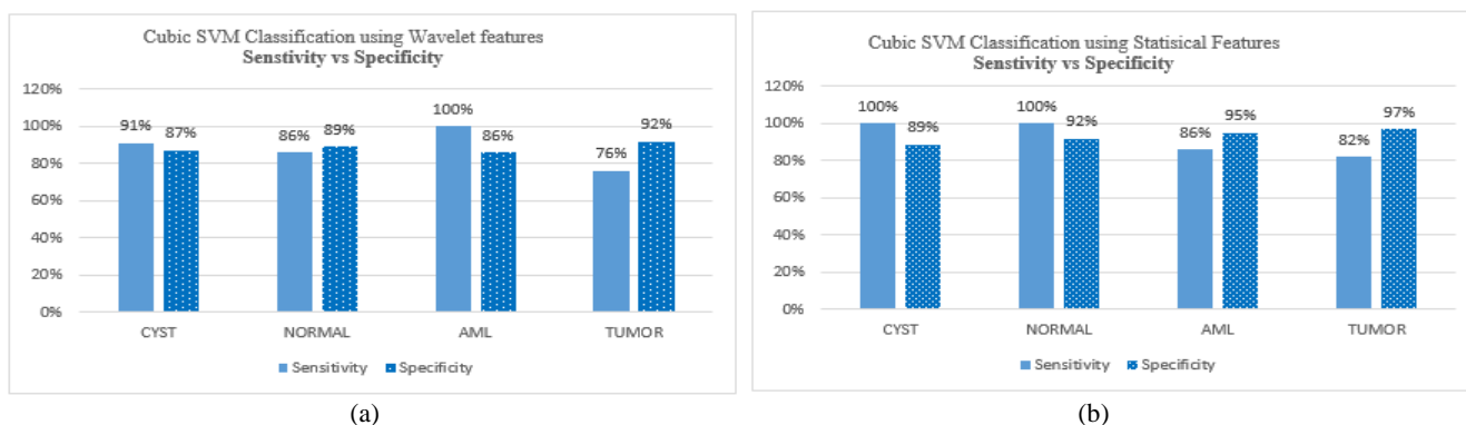
Fig 6: Comparison of Sensitivity and Specificity for a) wavelet features b) statistical features using Cubic SVM classifier
