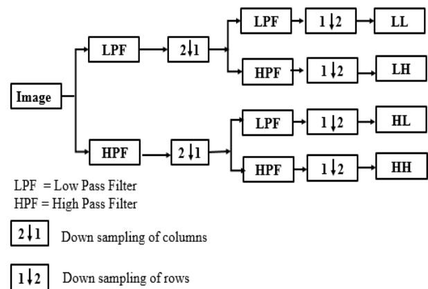
Fig 2:2D Discrete Wavelet Transform
