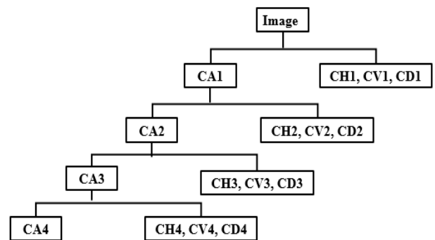
Fig 3: DWT decomposition – Four Level
