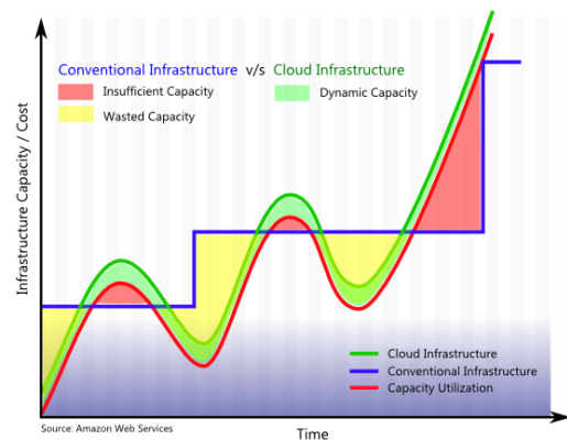
Fig. 2: Infrastructure capacity /cost
