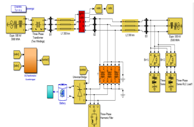
Fig. 7: System Model for Simulation.
