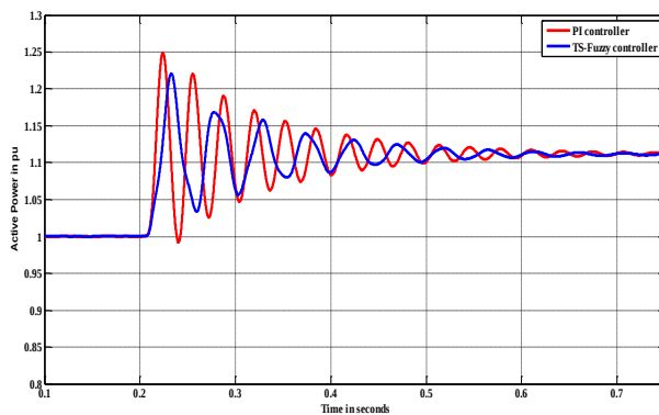
Fig. 10: The Step Change Response for Two Types of Controlle.
