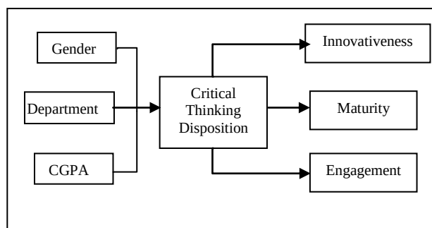
Fig 1: Theoretical Framework
