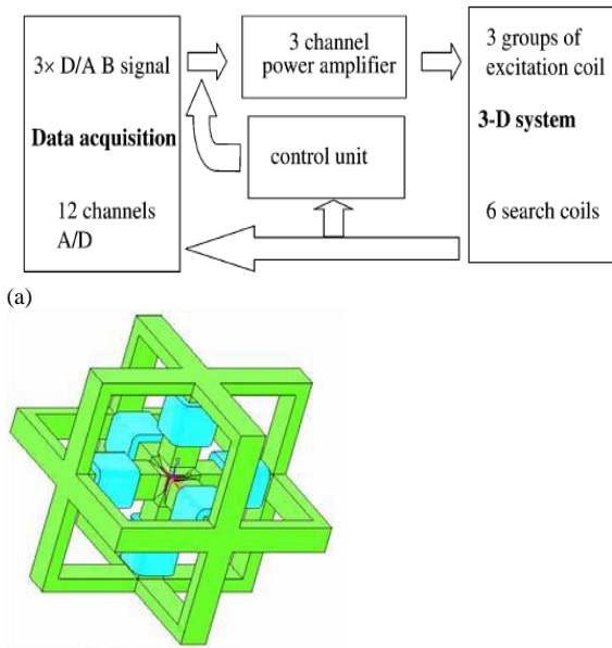
Fig. 1(a): 3-D tester (8) (b) Framework of 3-D tester (2).
