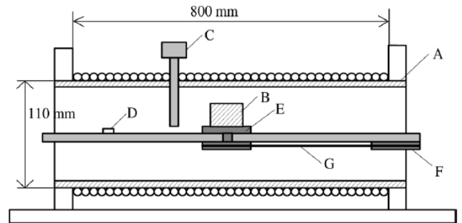
Solenoid: N=939 (turns), and H/l=1162.8 (1/m)
