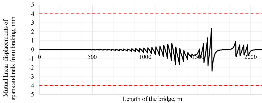
Fig. 7. Mutual linear displacements of spans and track under the braking load on the bridge across Kliazma river on HSR "Moscow - Kazan"
