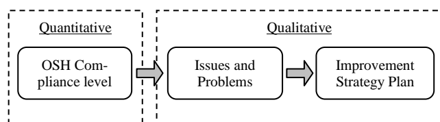
Fig. 1: Study Framework
