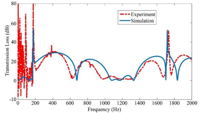
Fig. 6: Transmission loss comparison between Transfer Matrix Method and Experimental result
