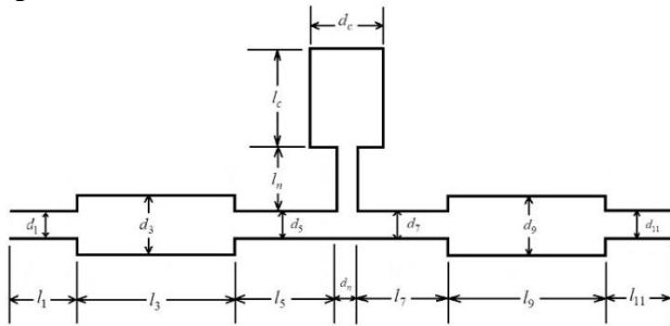
Fig. 5: Design parameters of the hybrid muffler: d_1, d_5, d_7, d_{11} = inlet and outlet pipes diameters of expansion chambers, d_3, d_9 = diameter of expansion chambers, d_c = diameter of Helmholtz Resonator cavity, d_n = diameter of neck of Helmholtz Resonator, l_1 = length of inlet pipes of front expansion chamber, l_3, l_9 = length of expansion chambers, l_5 = length of outlet pipe of front expansion chamber, l_n = length of neck of Helmholtz Resonator, l_c = length of Helmholtz Resonator cavity, l_7 = length of inlet pipe of rear expansion chamber, l_{11} = length of outlet pipe of rear expansion chamber
