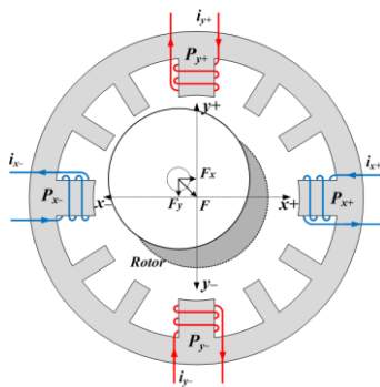
Fig. 2: Control of suspension force
