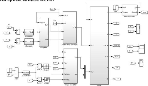
Fig.8: Simulink model of BLSRM system
