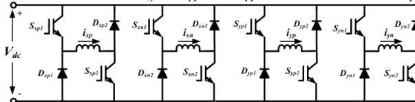
Fig. 3: H-bridge converter for suspension windings
