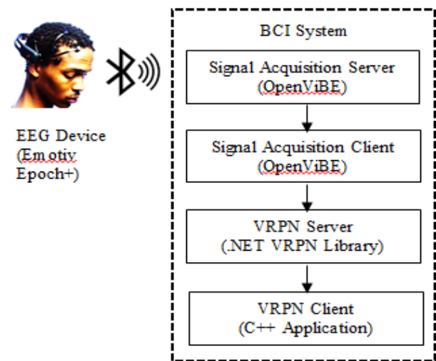
Fig. 6: BCI Architecture.
