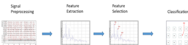
Fig. 3: Signal Processing Module of SSVEP BCI System.
