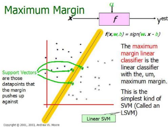
Fig. 5: Linear Support Vector Machines (LSVM).
