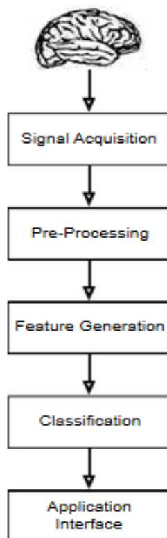
Fig. 1: BCI Framework.
