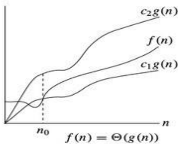
Fig.3: Theta notation
